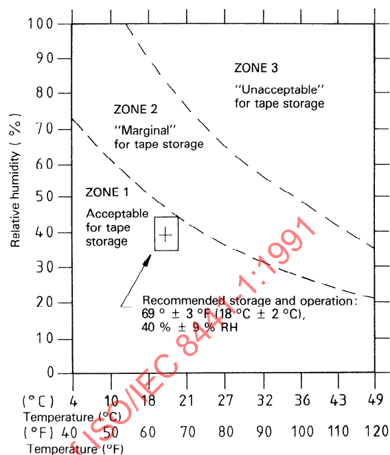
Figure C.1 — Contours of constant long-term storage environment
