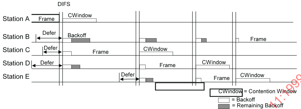
Figure 52—Backoff procedure
