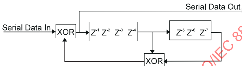
Figure 89—Data scrambler
