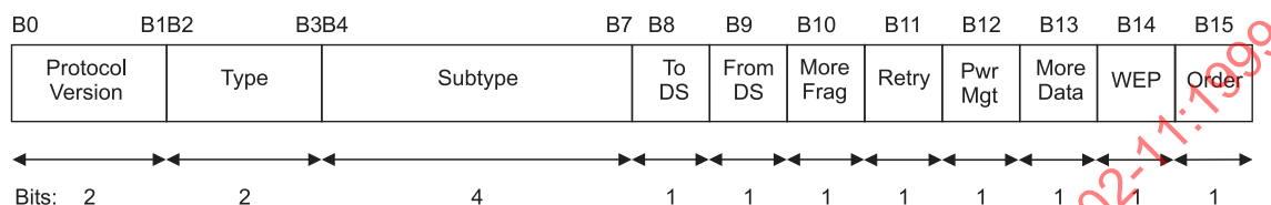
Figure 13—Frame Control field
