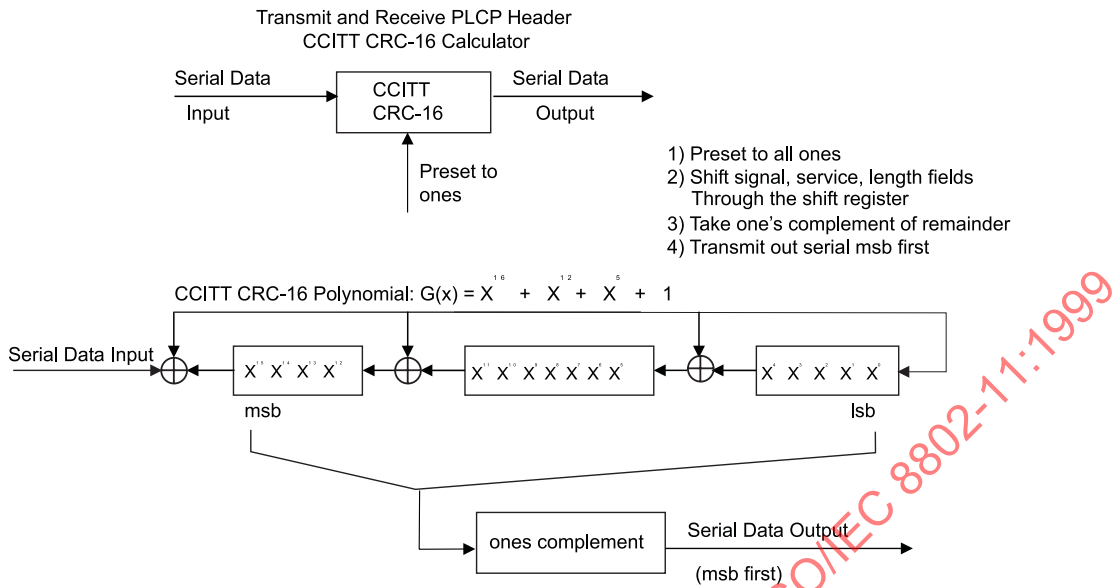
Figure 87—CCITT CRC-16 implementation
