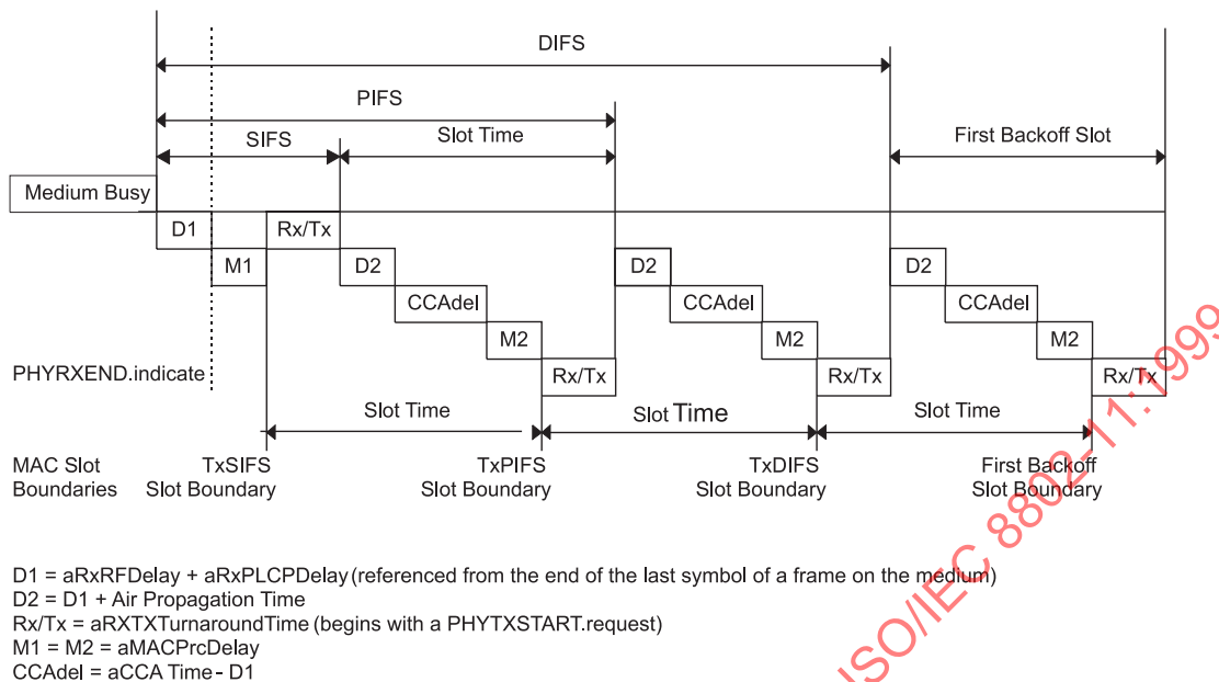
Figure 58—DCF timing relationships
