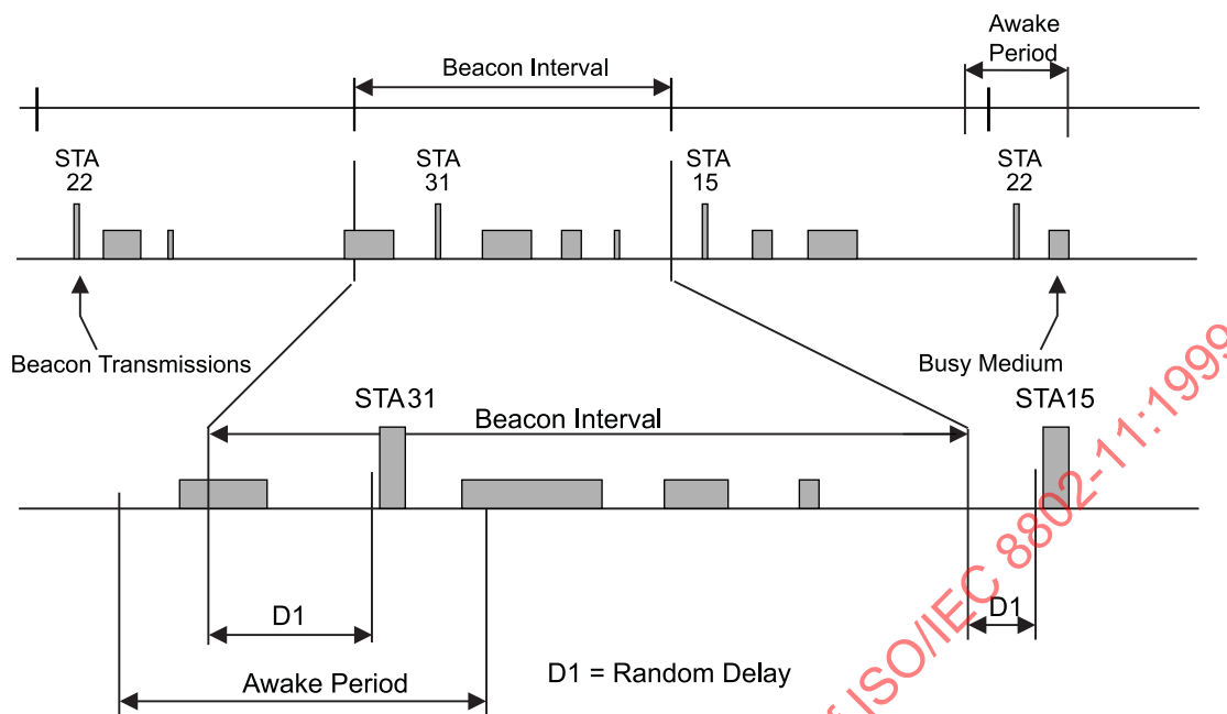
Figure 65—Beacon transmission in an IBSS
