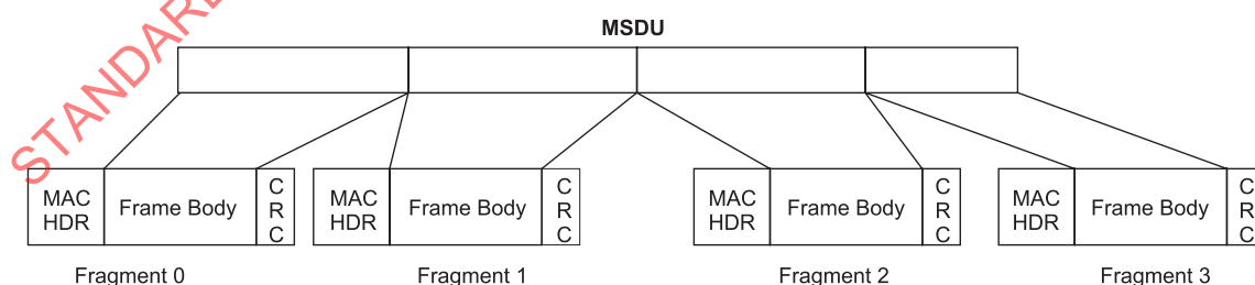
Figure 48—Fragmentation
