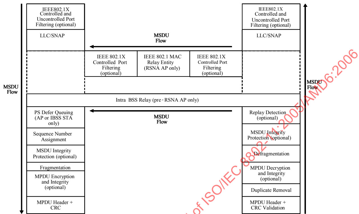
Figure 11g—MAC data plane architecture
