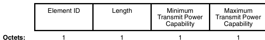
Figure 46b—Power Capability element format
