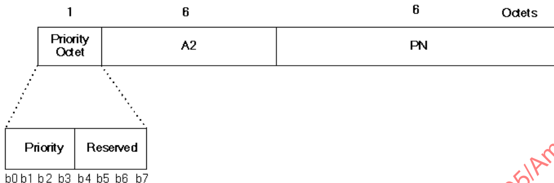
Figure 43q—Nonce construction
