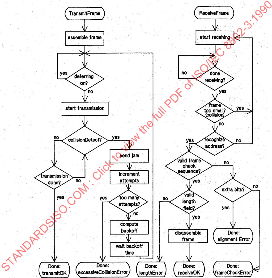
Fig 4-4 Control Flow Summary
