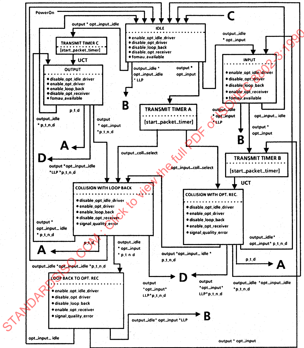
Fig 9-8 FOMAU Transmit, Receive, and Collision Functions State Diagram
