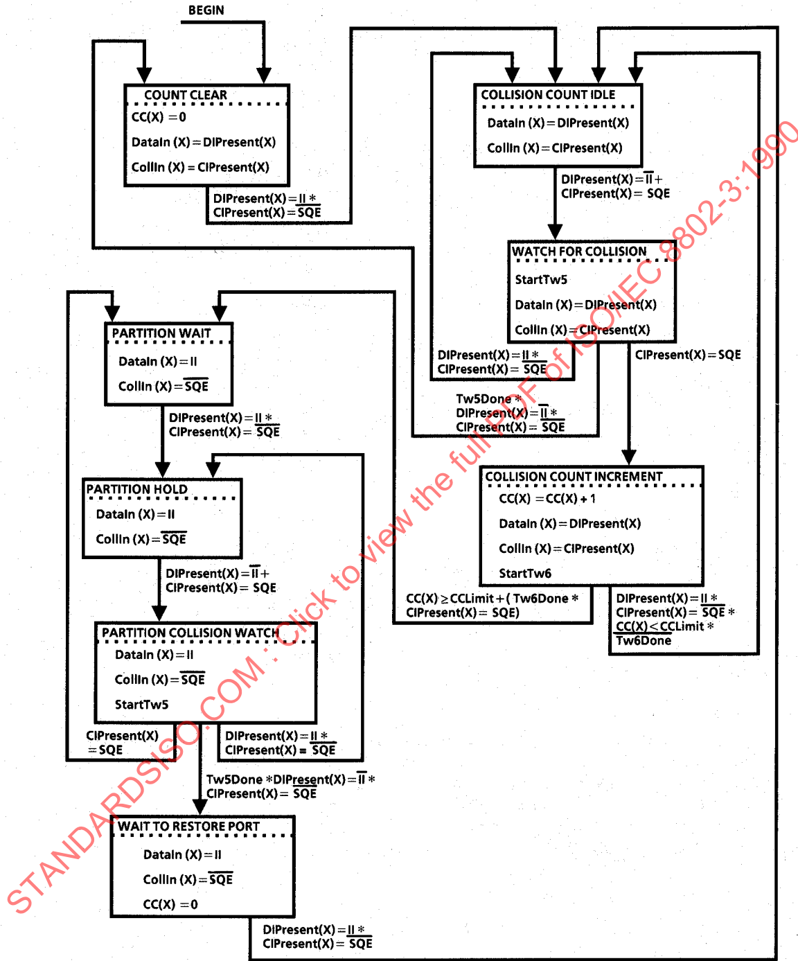
Fig 9-6 Partitioning State Diagram for Port X
