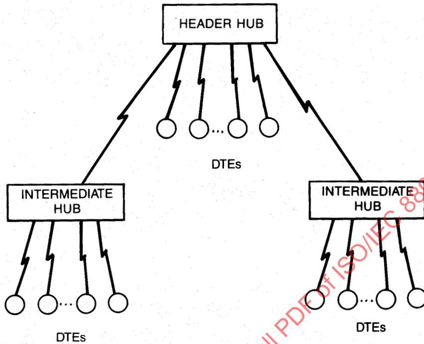
12-3 Network With Two Levels of Hubs
