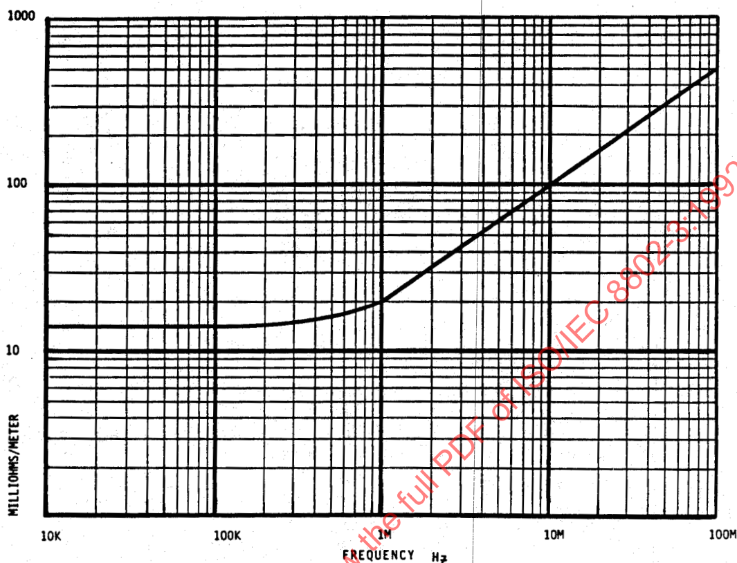
Fig 10-6 Maximum Coaxial Cable Transfer Impedance
