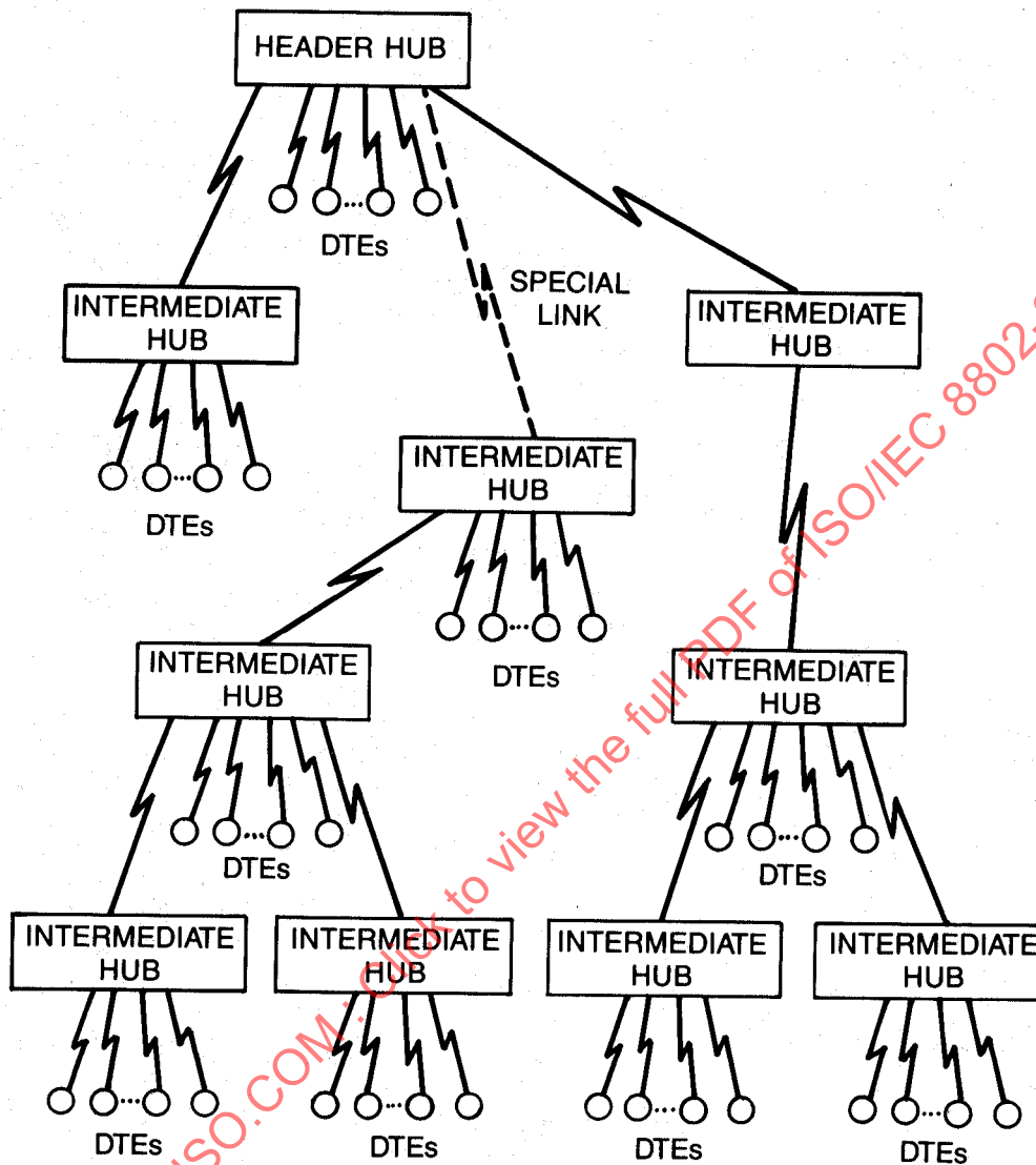
Fig 12-4 Network With Four Levels of Hubs
