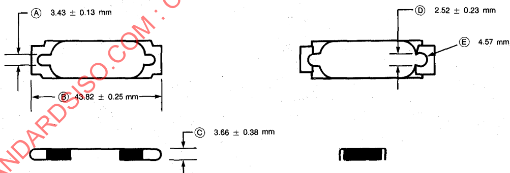
Fig 7-19 Connector Slide Latch (material 24 gauge maximum)
