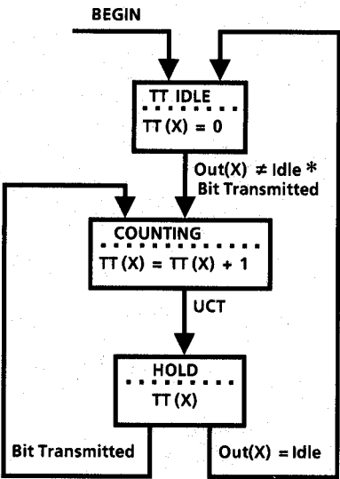
Fig 9-3 Transmit Timer State Diagram for Port X
