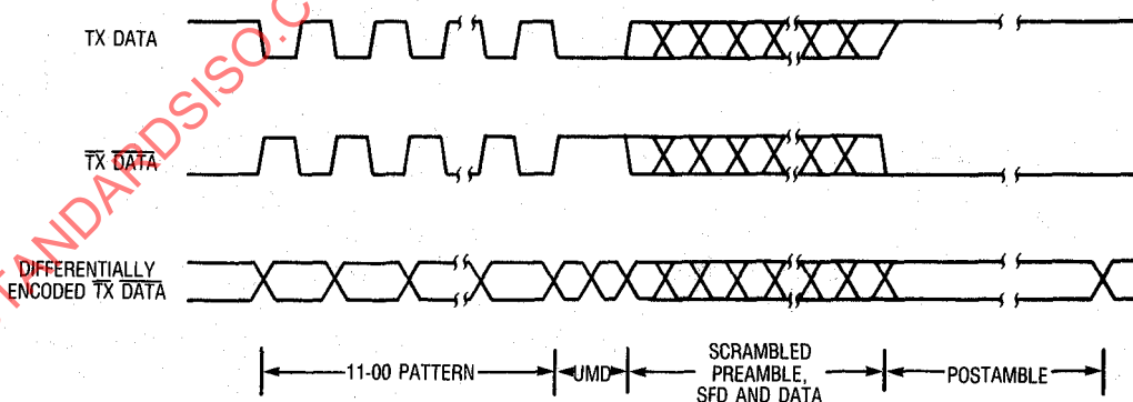
Fig 11-9 Packet Format at Modulator Input
