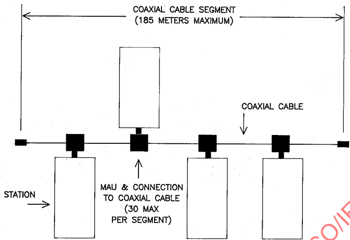
Fig 10-9 The Minimum System Configuration
