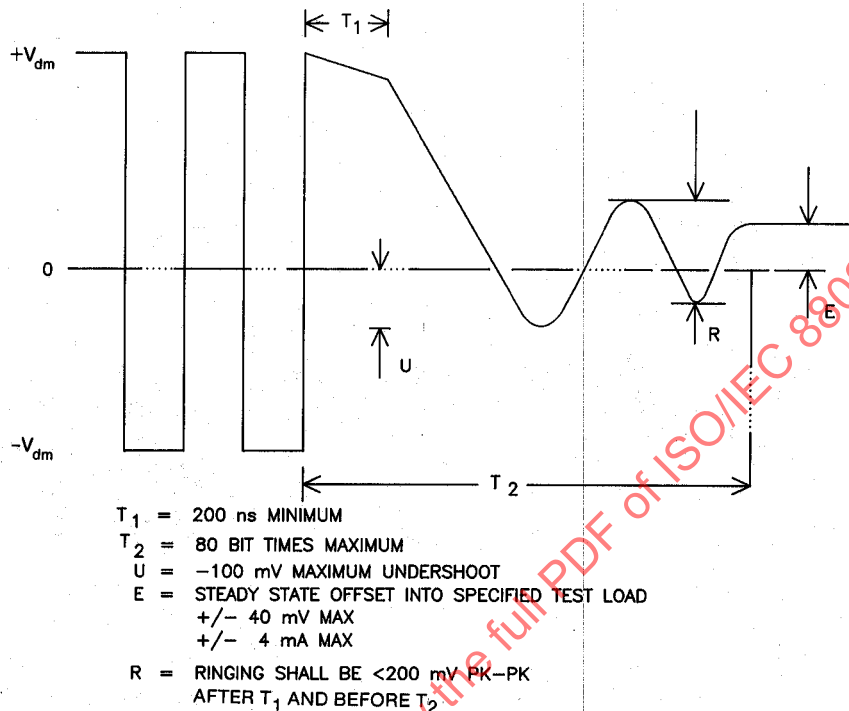
Fig 7-12 Generalized Driver Waveforms
