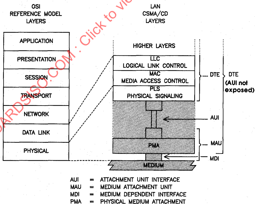
Fig 10-1 Physical Layer Partitioning; Relationship to the ISO Open System Interconnection (OSI) Reference Model
