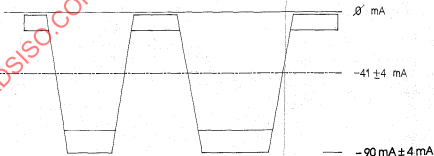
Fig 10-4 Driver Current Signal Levels
