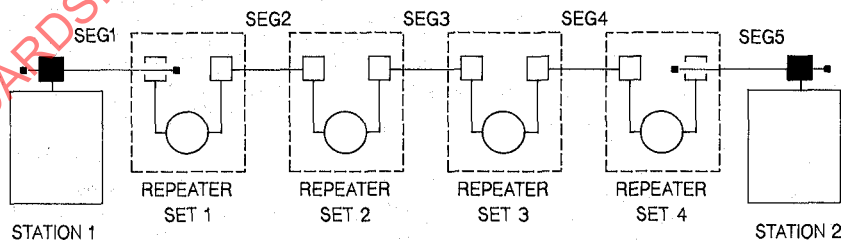
Fig 10-8 Maximum Transmission Path
