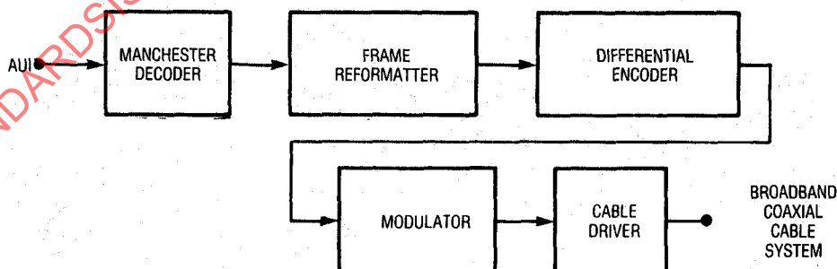
Fig 11-3 Transmit Function Requirements
