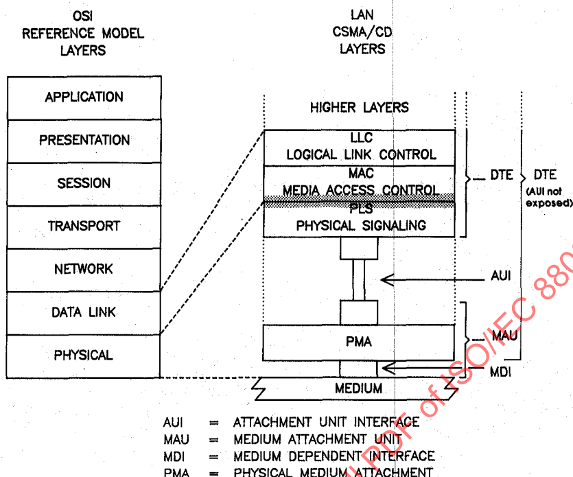
Fig 6-1 Service Specification Relationship to the LAN Model
