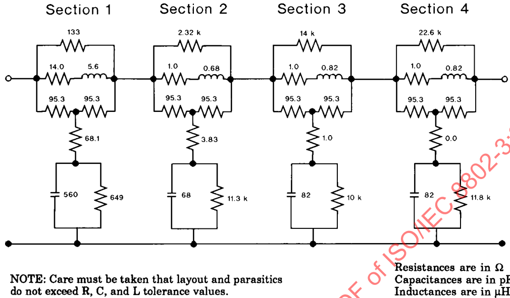
Figure 14-7—Twisted-pair model
