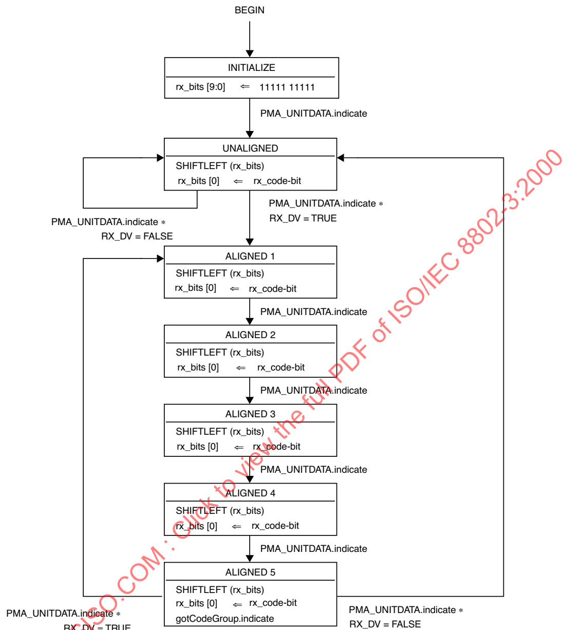
Figure 24–10—Receive Bits state diagram
