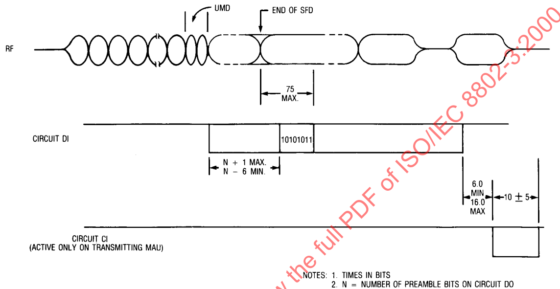
Figure 11–13—No collision timing diagram (coax to AUI)
