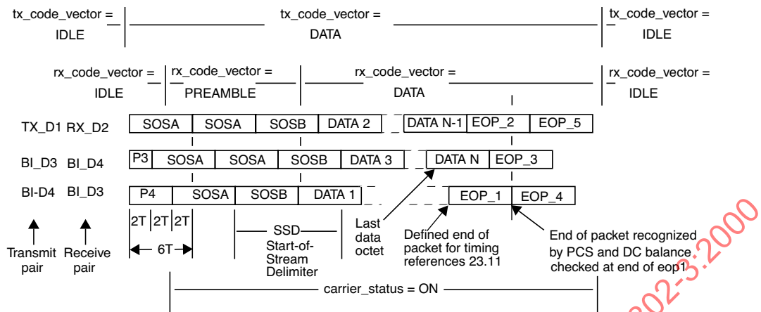
Figure 23-6—PCS sublayer to PMA sublayer frame structure
