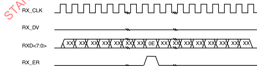
Figure 35–12 — False Carrier indication
