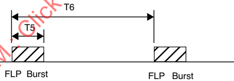
Figure 28-6—FLP Burst to FLP Burst timing
