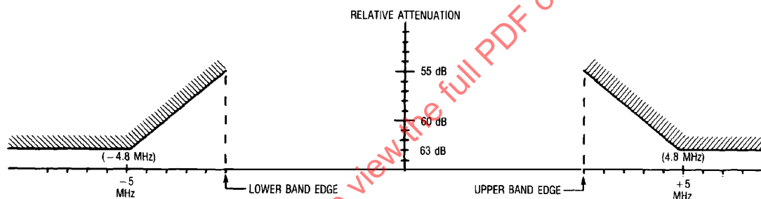
Figure 11–8—Transmit out-of-band power attenuation
