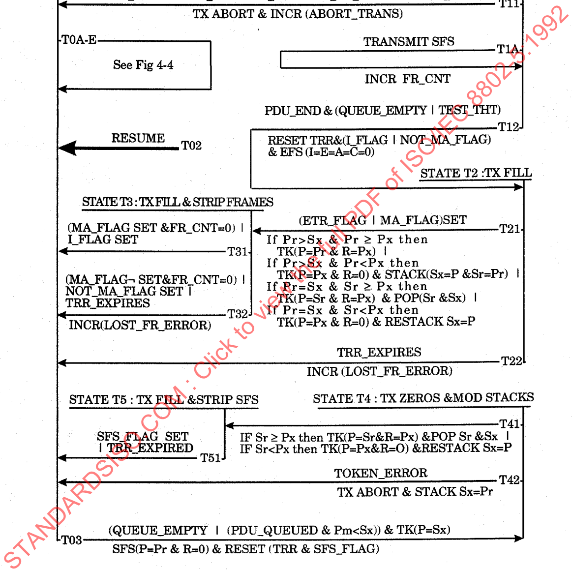
Operational Finite-State Machine Diagram
