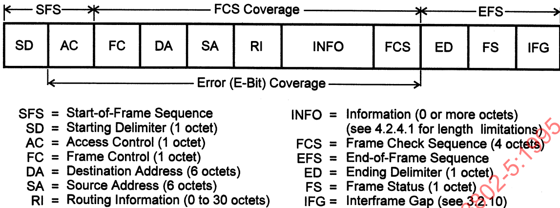
Figure 6—Frame format
