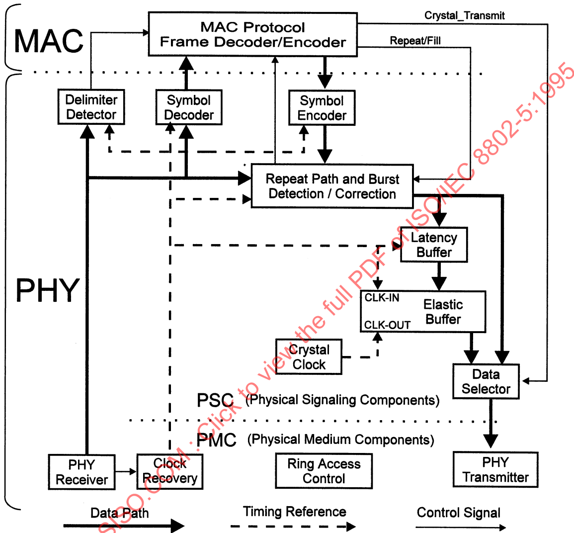
Figure 26—Station data path example
