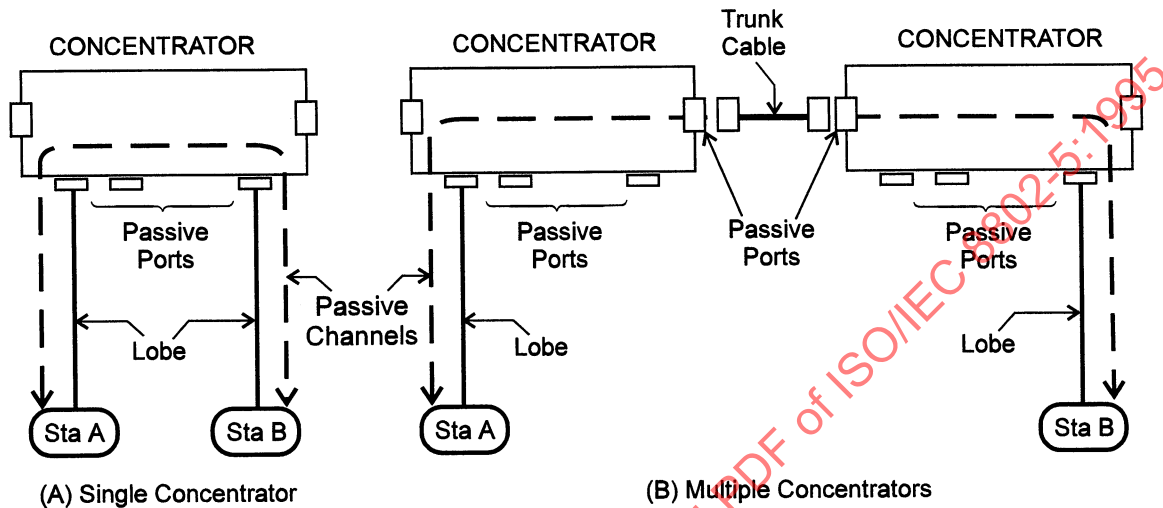
Figure 37—Passive channel 18
