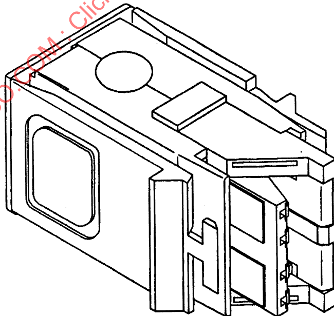
Figure 43—MIC_S—isometric view
