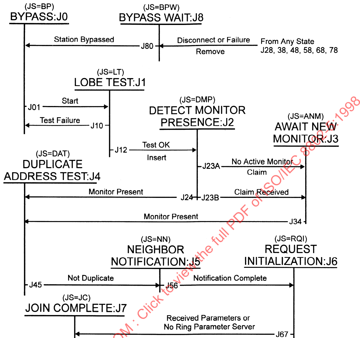
Figure 23—Join Ring FSM diagram
