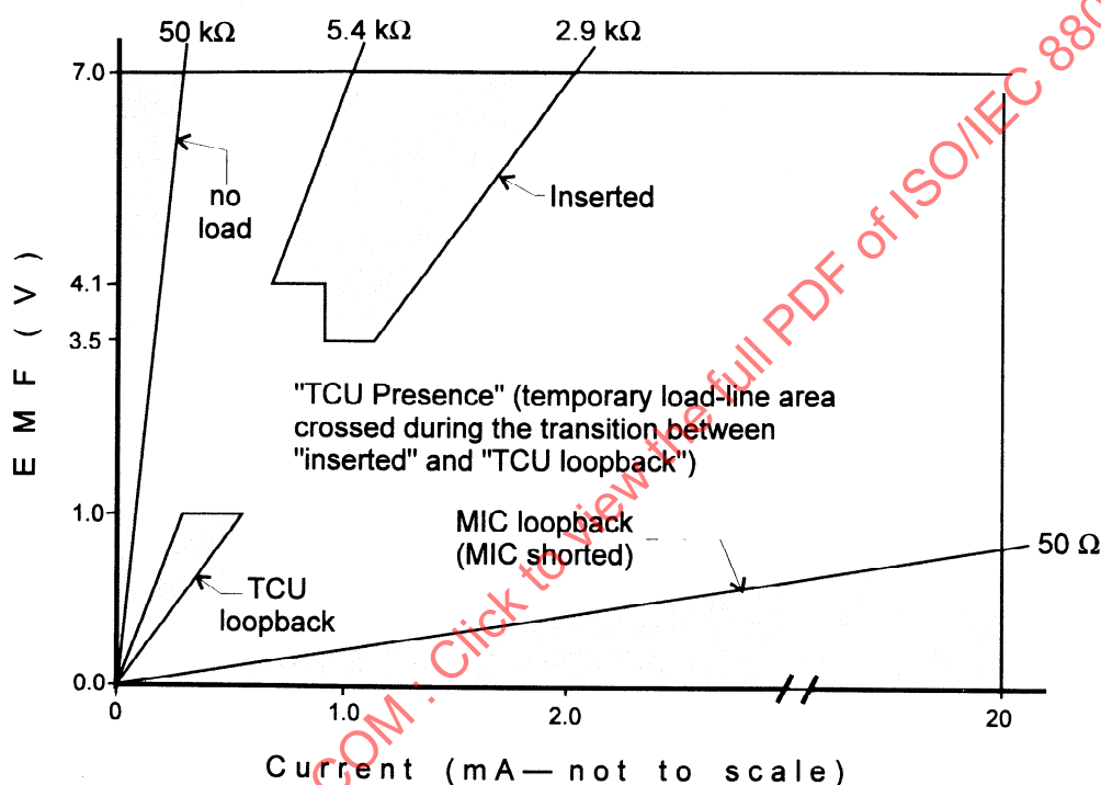
Figure 31—Operating regions for compliant load conditions
