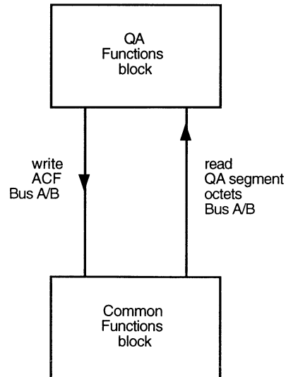
Figure 5-26—Receive interaction between Common Functions block and QA Functions block
