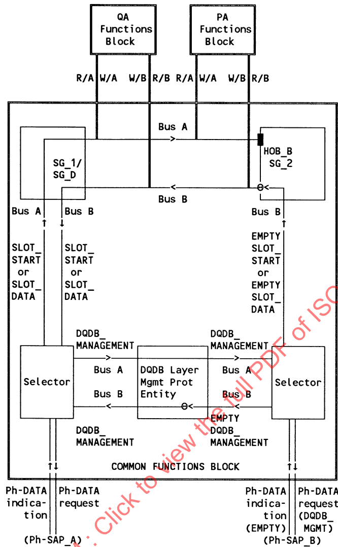
Figure 5-35—Functional data path for node performing Head of Bus B function
