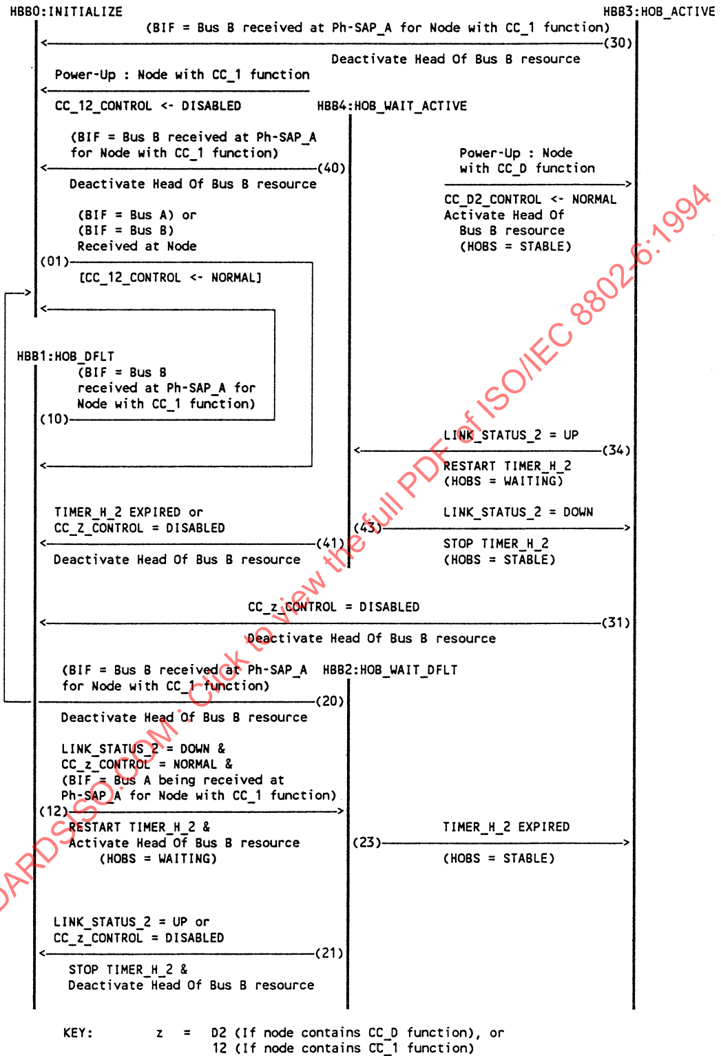
Figure 10-7—Head of Bus State Machine transition diagram (CC_function)
