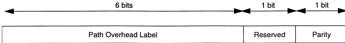
Figure 16-2—POI octet
