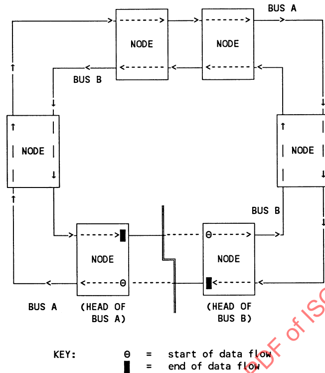
Figure 2-12—Subnetwork reconfiguration
