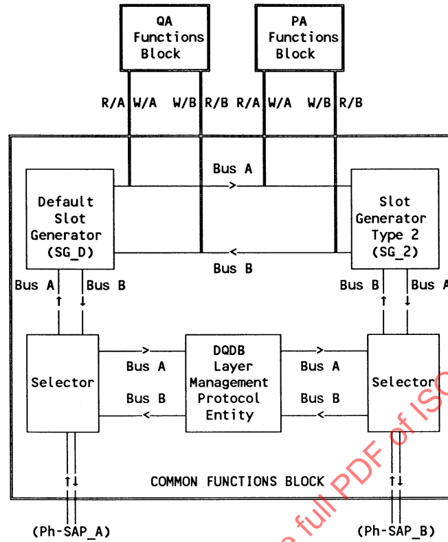
Figure 5-29—Slot generator designations for the node supporting the Default Slot Generator function
