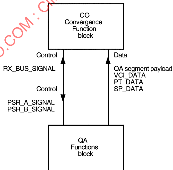
Figure 5-22—Receive interaction between QA Functions block and COCF block
