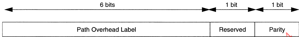
Figure 14-2—POI octet
