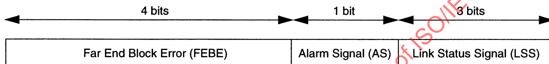
Figure 14-3—PLCP Path status (G1)
