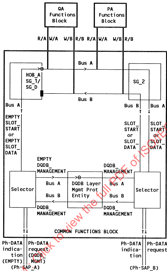
Figure 5-34—Functional data path for node performing Head of Bus A function
