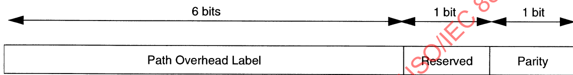
Figure 13-2—POI octet
