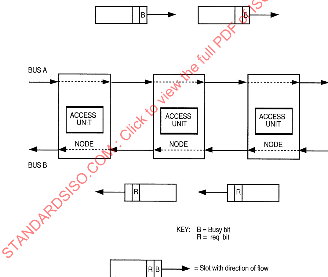
Figure 2-3—Queue formation on Bus A
