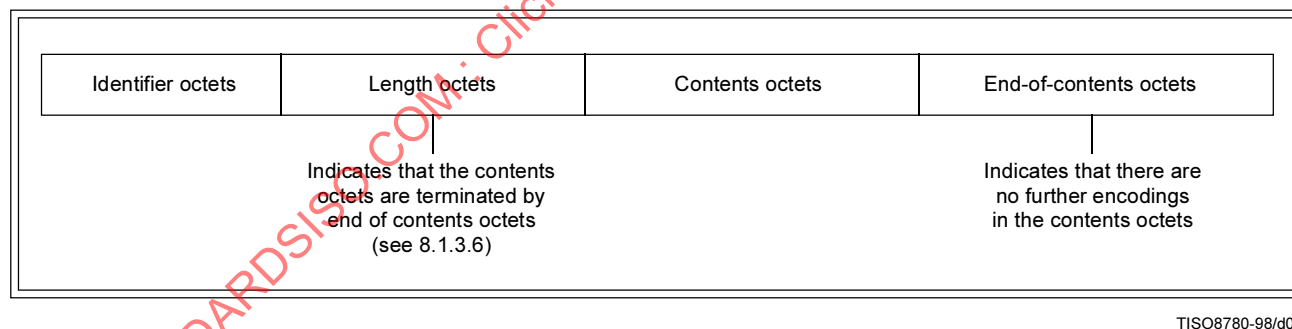
Figure 2 – An alternative constructed encoding
