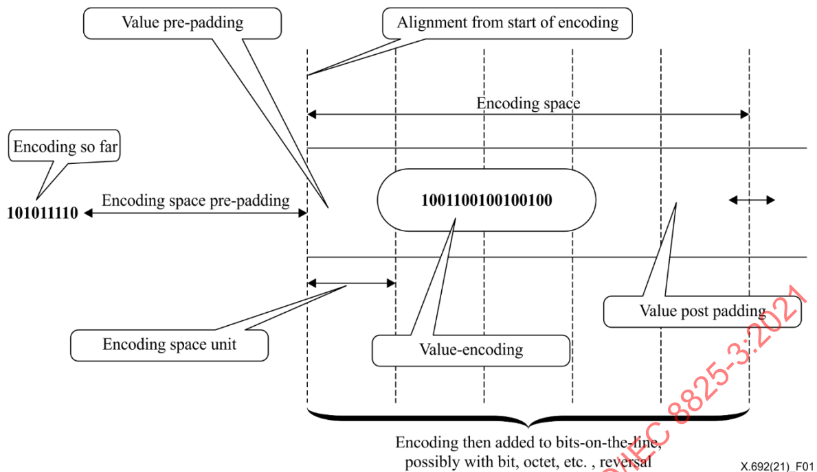
Figure 1 – Encoding space, value-encoding and padding concepts
