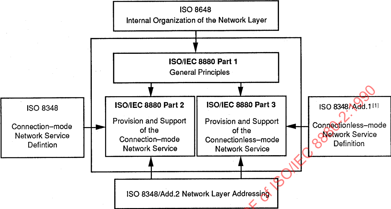
Figure 1 – Organization of ISO/IEC 8880
