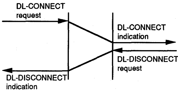
Figure 11 - Sequence of primitives in a DLS User rejection of a DLC establishment attempt.
