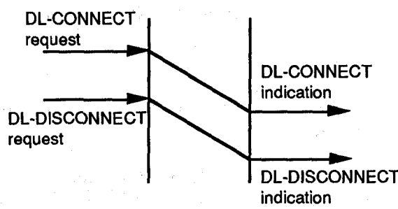
Figure 14 - DL-DISCONNECT indication arrives before DL-CONNECT response is sent
