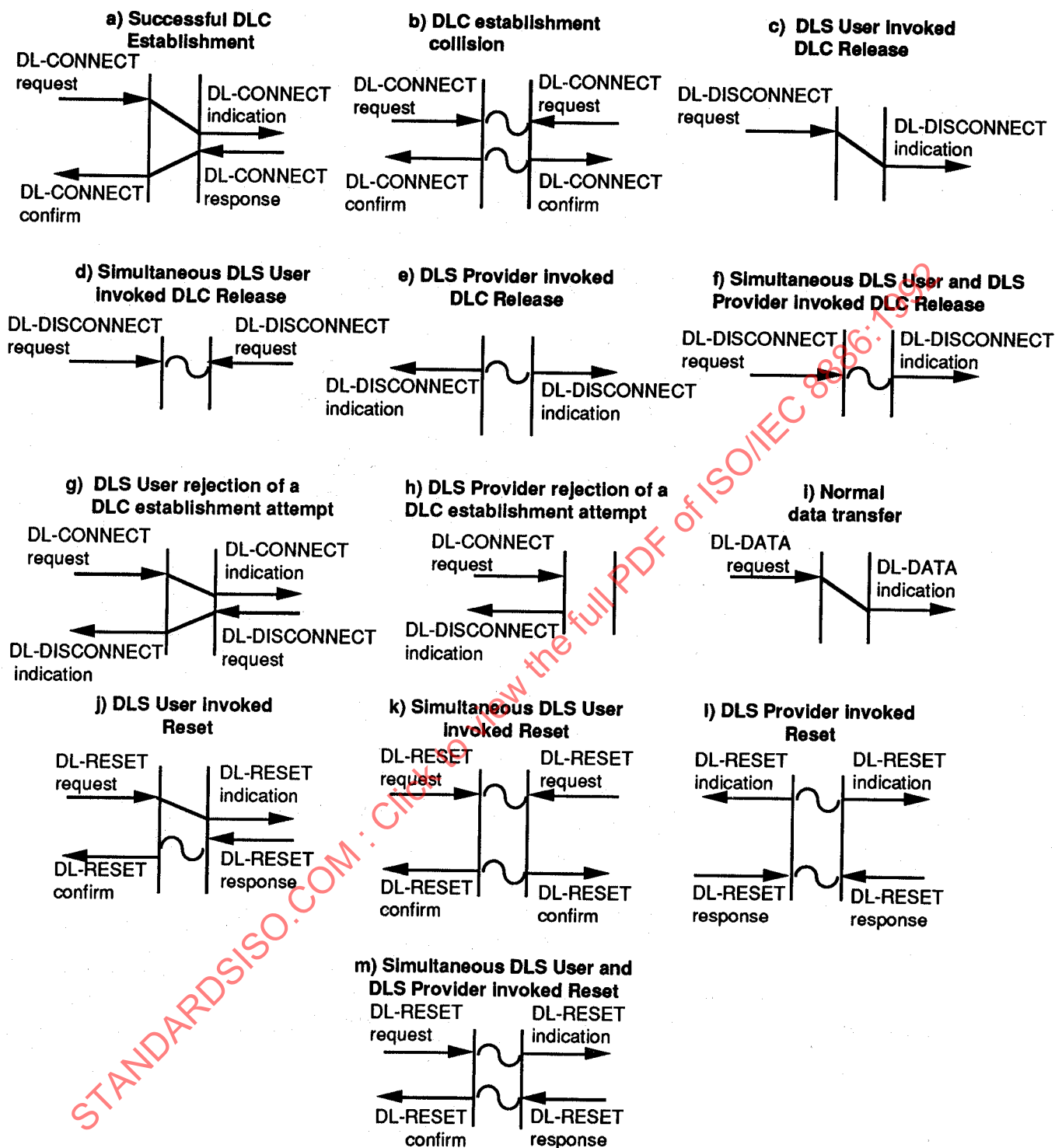
Figure 4 - Summary of Data-link-connection-mode service primitive time-sequence diagrams
