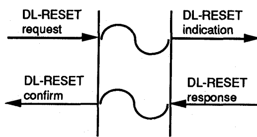
Figure 20 - Sequence of primitives in a simultaneous DLS User and DLS Provider initiated Reset Service
