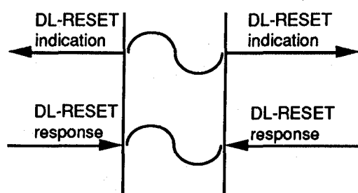
Figure 19 - Sequence of primitives in a DLS Provider initiated Reset Service
