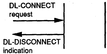
Figure 12 - Sequence of primitive in DLS Provider rejection of a DLC establishment attempt
