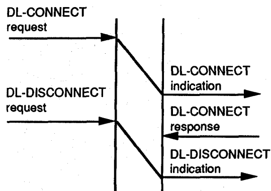
Figure 15 - DL-DISCONNECT indication arrives after DL-CONNECT response is sent
