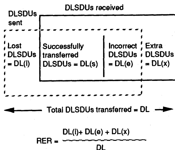
Figure 3 - Components of Residual Error Rate
