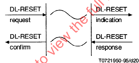
Figure 19 – Sequence of primitives in a simultaneous DLS user and DLS provider initiated reset service
