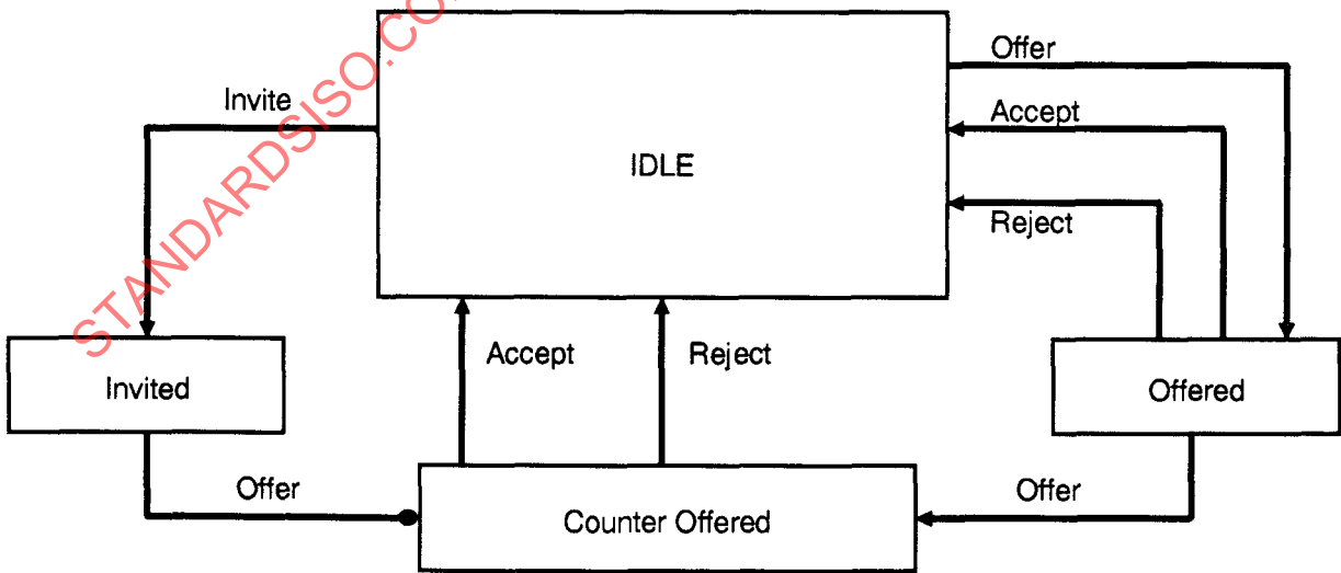
Figure A.1 - Negotiation state diagram
