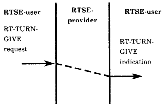
Figure 6 - RT-TURN-GIVE service-primitives
