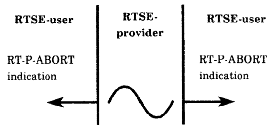
Figure 7 - RT-P-ABORT service-primitives
