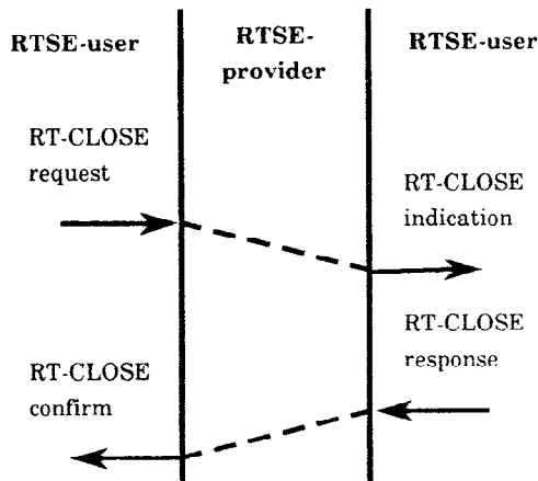
Figure 3 - RT-CLOSE service-primitives
