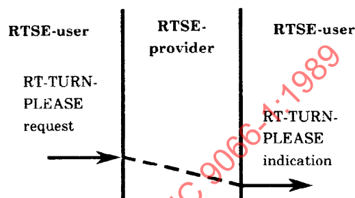
Figure 5 - RT-TURN-PLEASE service-primitives
