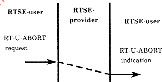
Figure 8 - RT-U-ABORT service-primitives
