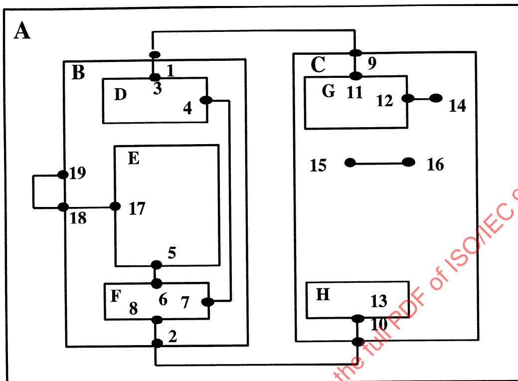
Figure D.3 - Module instances and their communication links.
