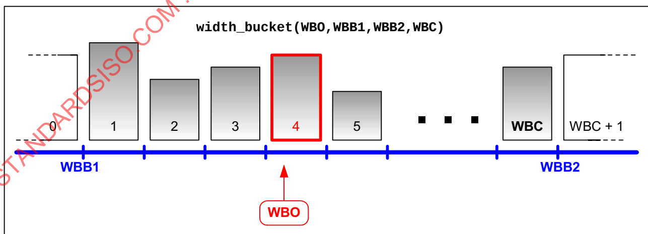
Figure 1—Illustration of WIDTH_BUCKET Semantics
