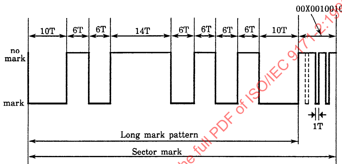
Figure 9 - Sector Mark pattern with negative polarity
