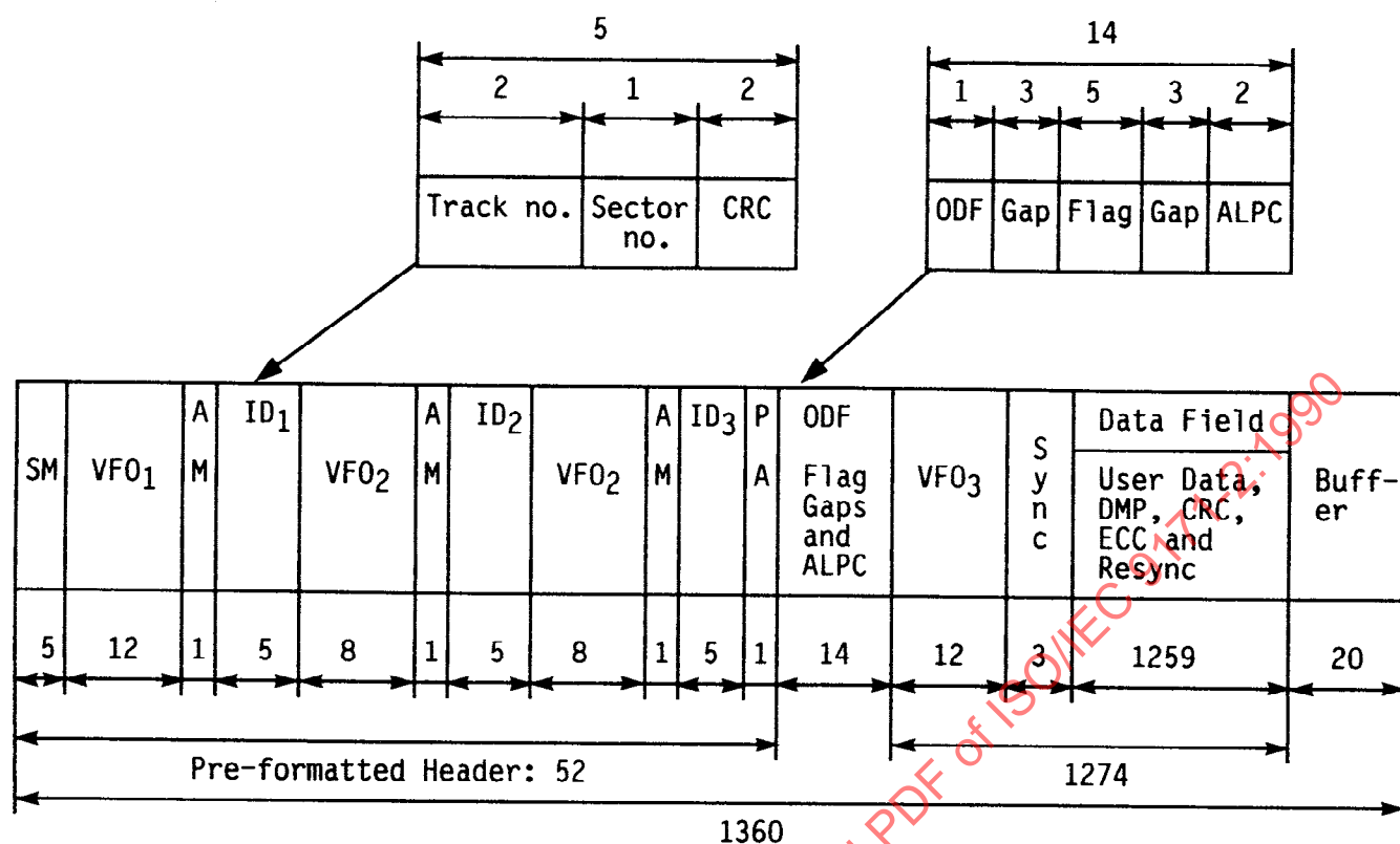
Figure 7 - Sector format for 1024 user bytes
