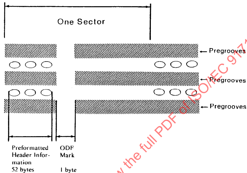
Figure 5 - Example of sector with offset detection flag for on-land recording (schematic)
