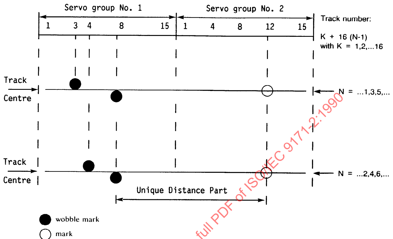
Figure 11 - Layout of the servo area
