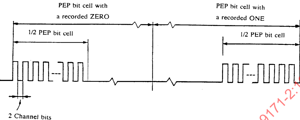
Figure 1 - Example of phase-encoded modulation in the PEP Zone
