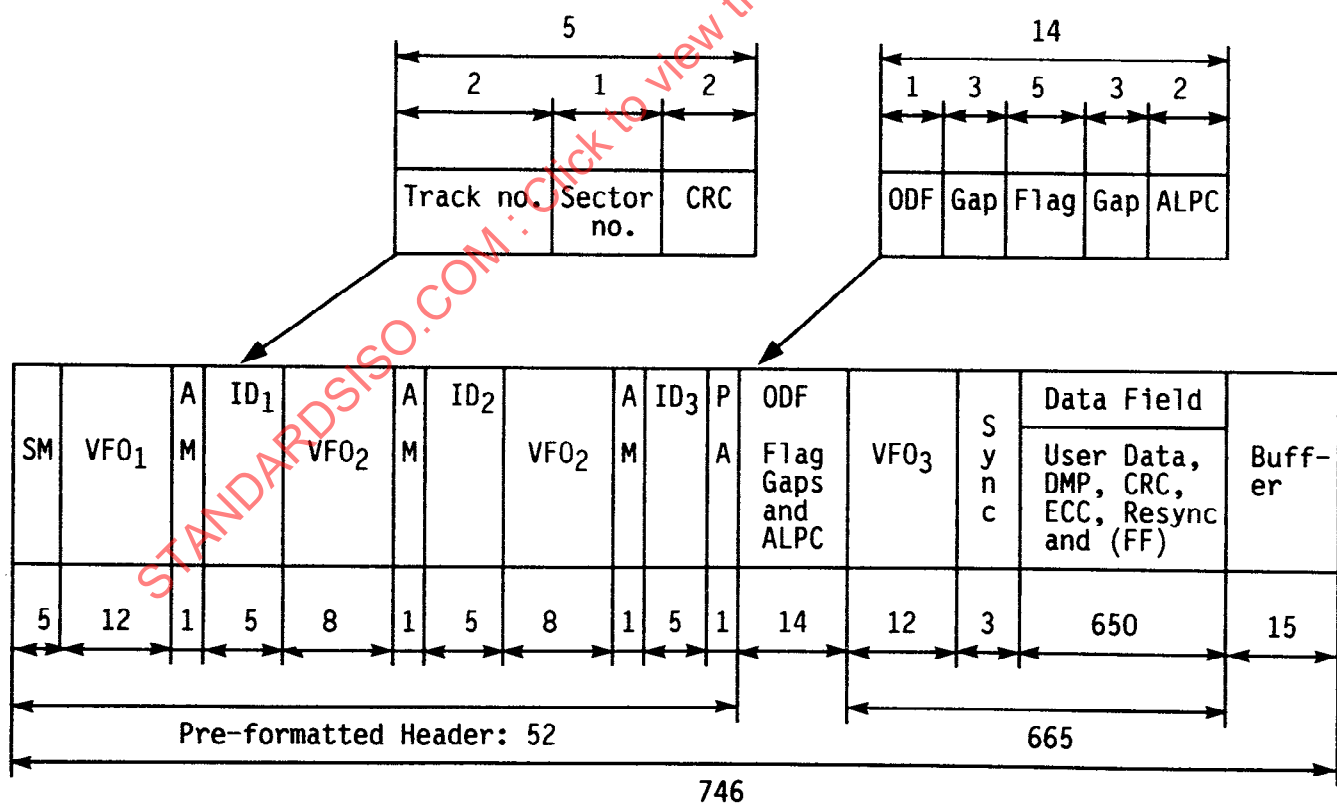
Figure 8 - Sector format for 512 user bytes
