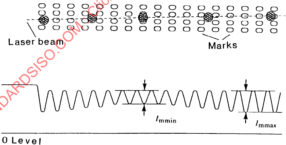
Figure 2 - Path of the laser beam crossing tracks, and the resulting PEP signals
