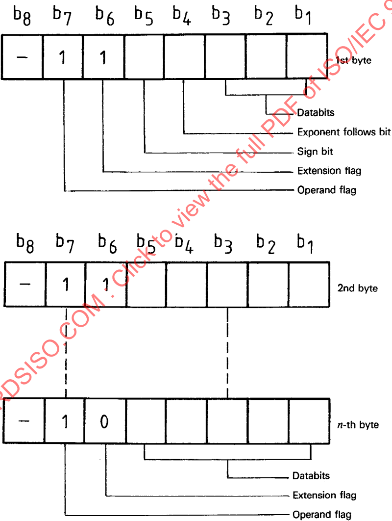
Figure 16 — Encoding of a mantissa using the basic format REAL EXPLICIT EXPONENT = ALLOWED
