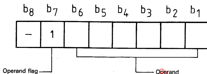
Figure 3 — Operand encoding structure
