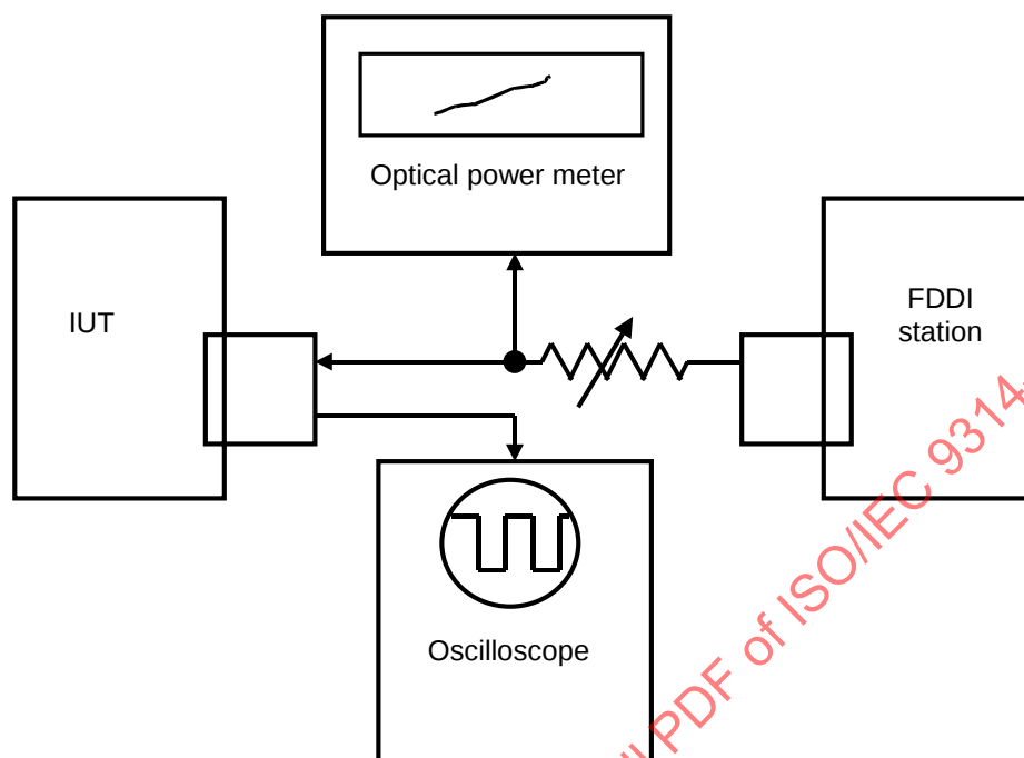
Figure 12 – Signal_Detect assertion
