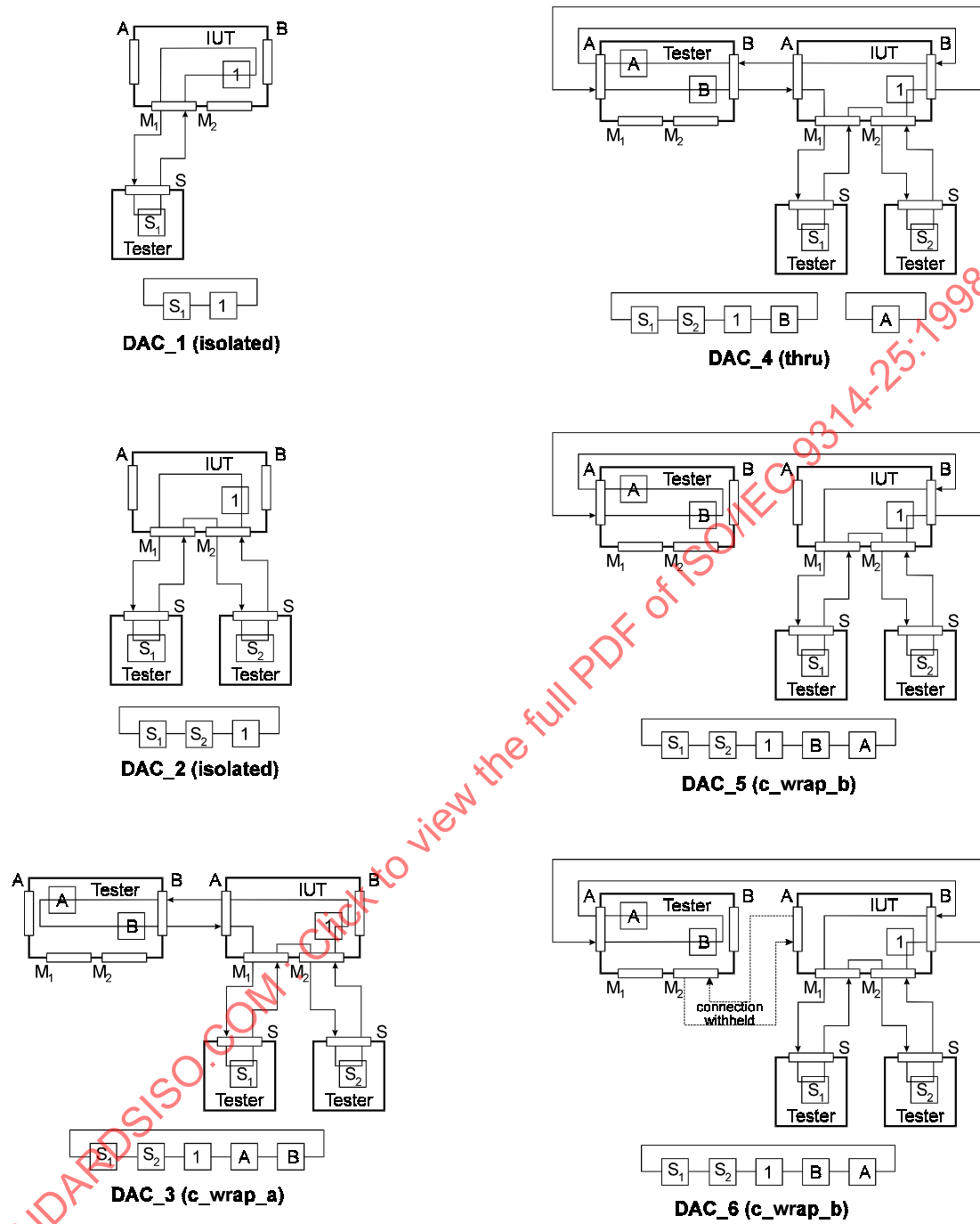
Figure 18 - Single MAC DAC Test Configurations (1 of 2)
