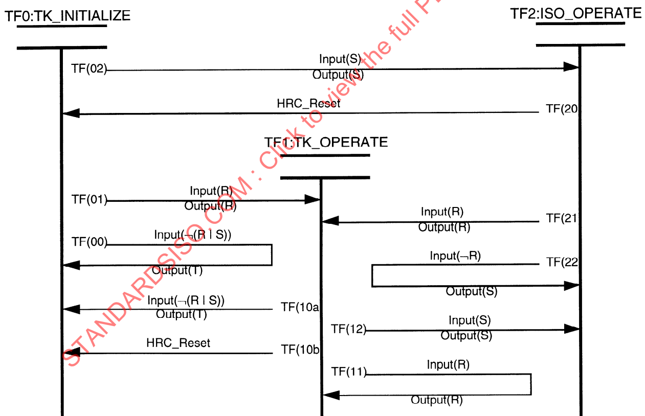
Figure 15 — WBC template filter state diagram
