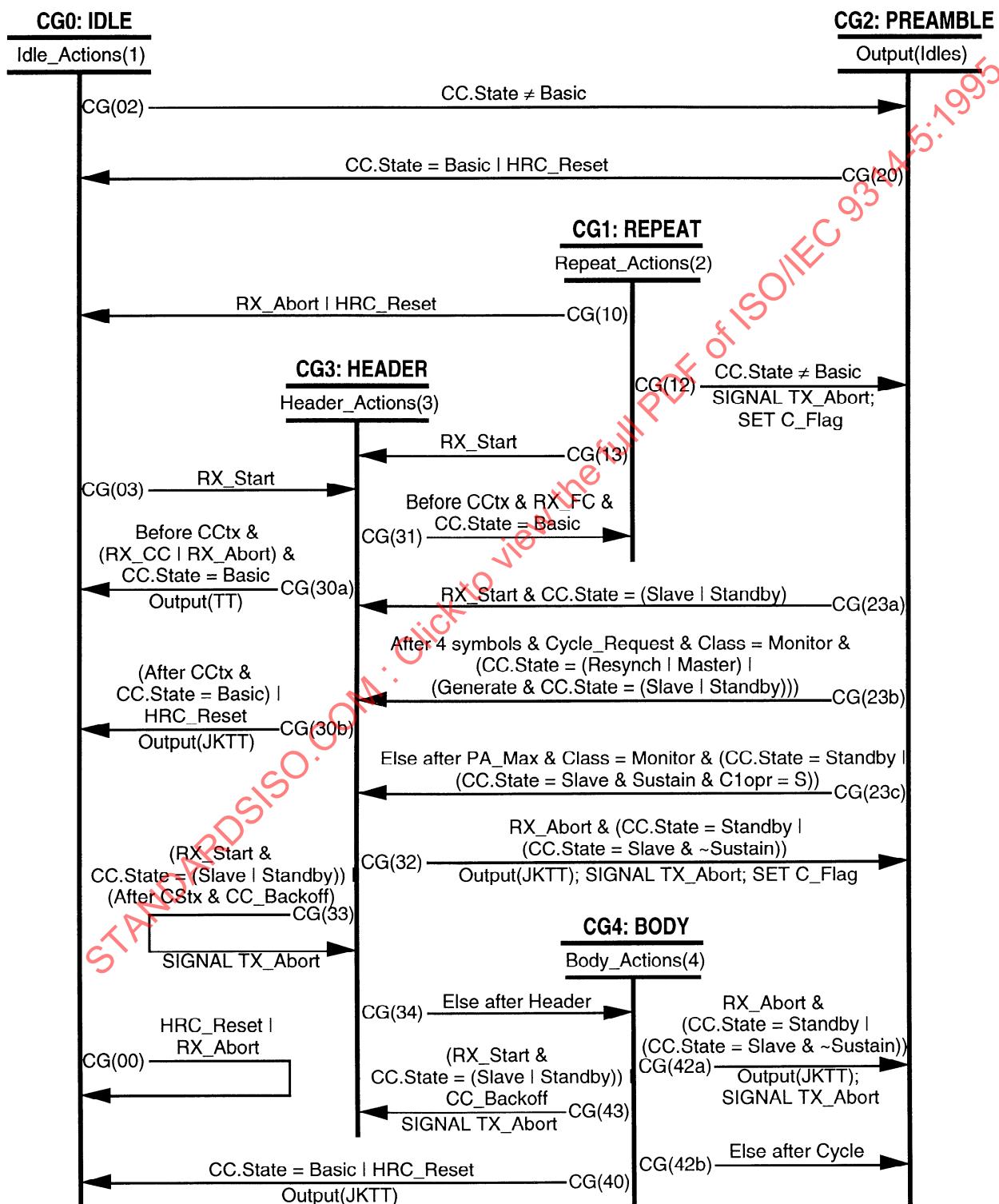
Figure 17 — HRC cycle generate state diagram (Part 1 of 4)
