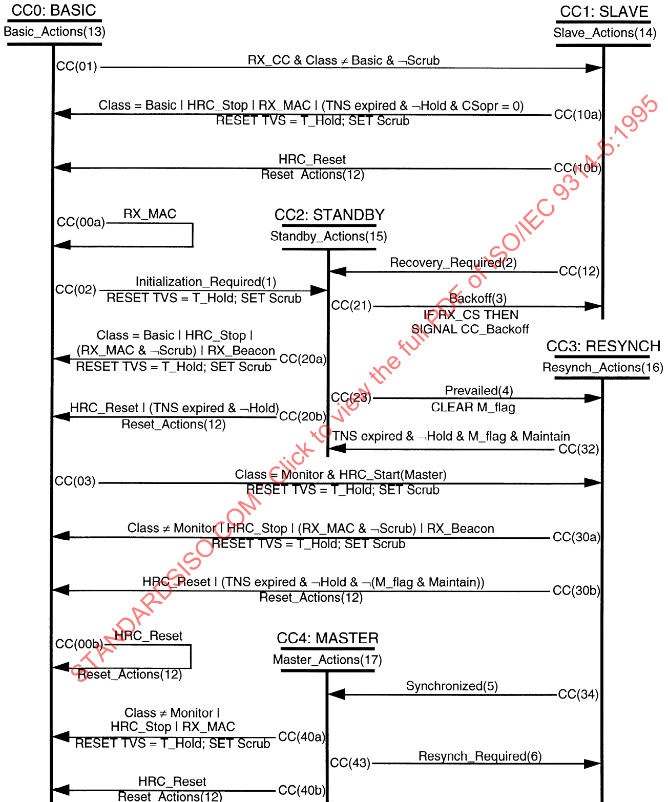
Figure 16 — HRC cycle control state diagram (Part 1 of 5)
