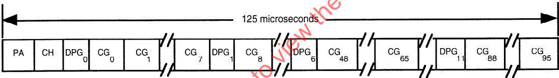
Figure 9 — H-MUX cycle structure at 100 Mbps
