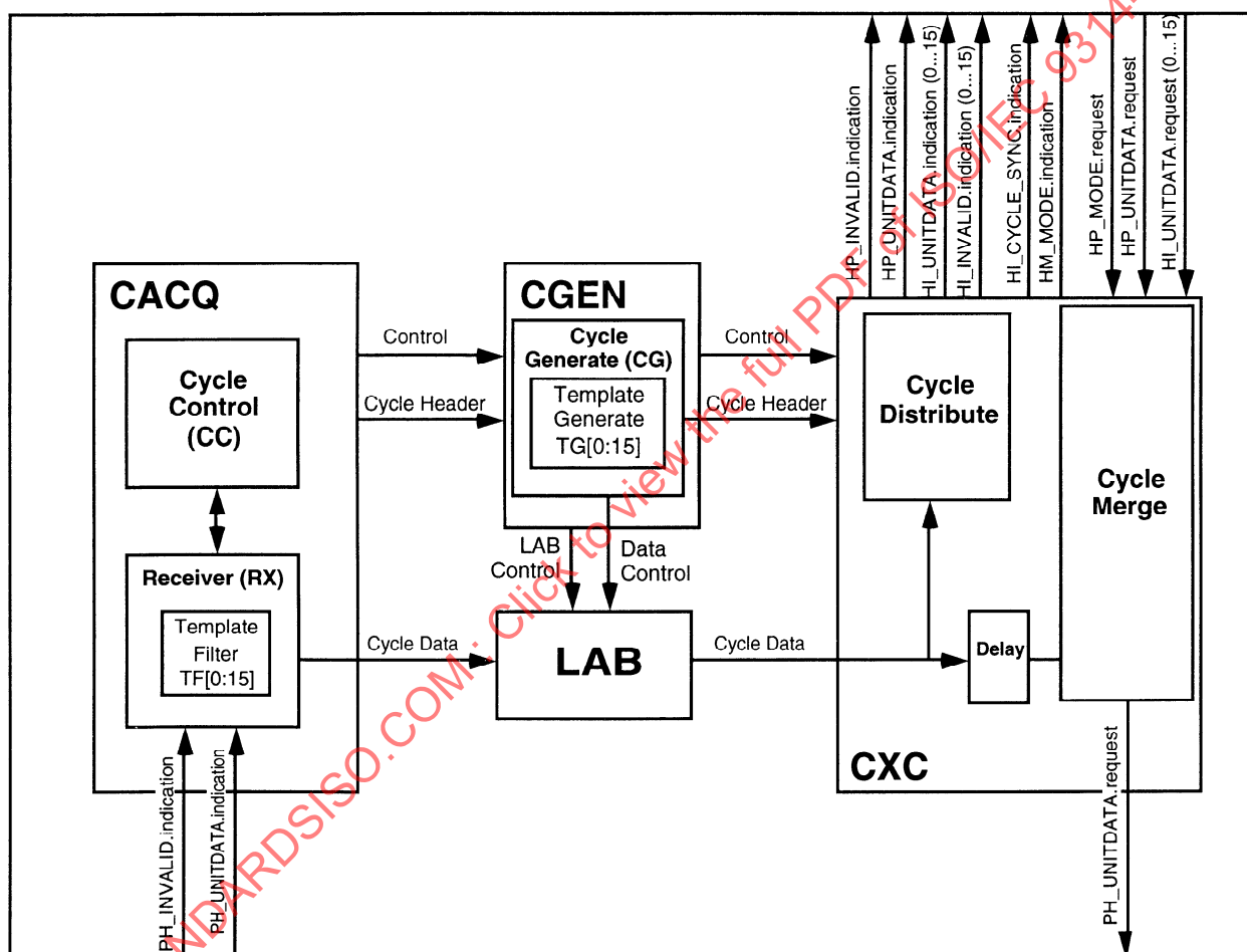
Figure 13 — H-MUX structure
