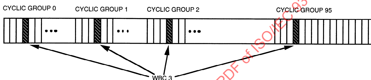
Figure 11 — Example of wideband channel interleaving
