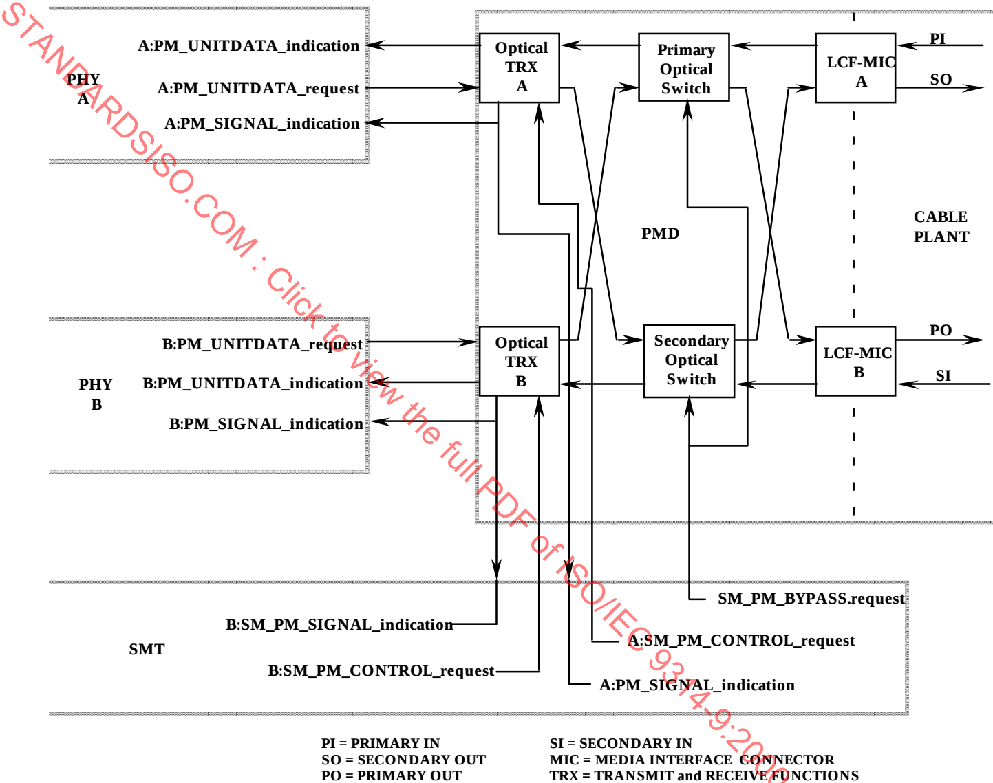
Figure 4 — Dual attachment LCF-PMD services
