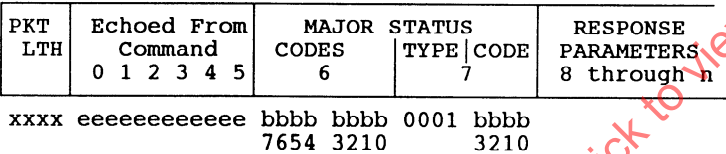
Figure 10 – Response packet for position control
