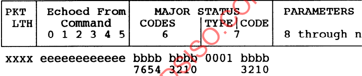
Figure 6 – Response packet for operating mode
