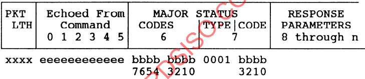
Figure 28 – Response packet for erase
