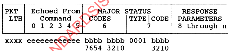
Figure 12 – Response packet for report position
