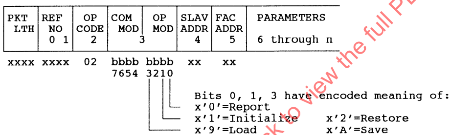
Figure 1 – Command packet for attributes
