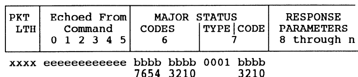
Figure 20 – Response packet for write
