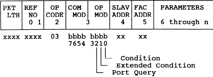
Figure 3 – Command packet for report addressee status
