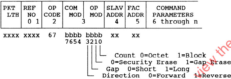
Figure 27 – Command packet for erase
