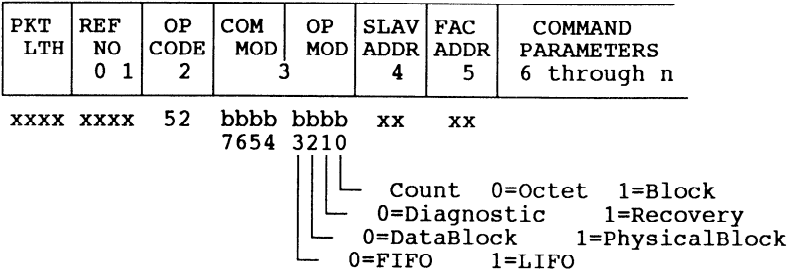
Figure 23 – Command packet for read from buffer
