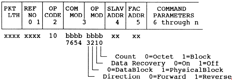
Figure 15 - Command packet for read
