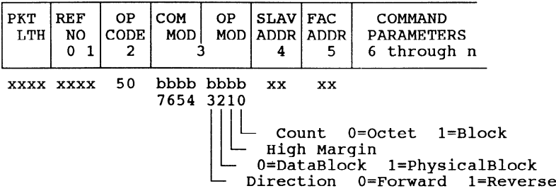
Figure 21 – Command packet for read verify
