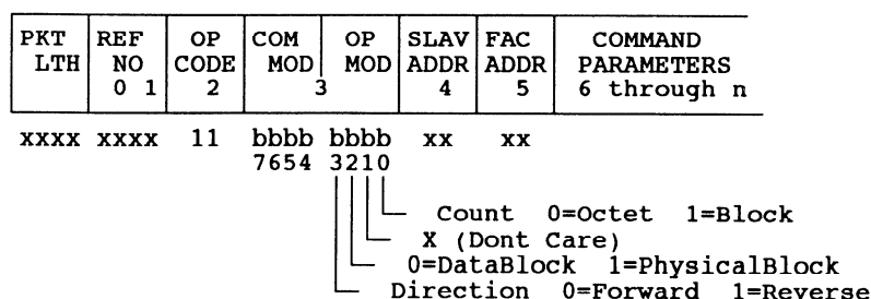
Figure 17 – Command packet for read raw data
