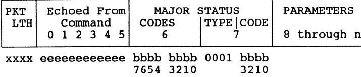
Figure 4 – Response packet for report addressee status
