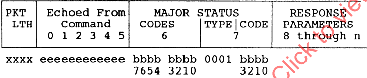
Figure 22 – Response packet for read verify
