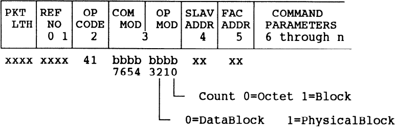
Figure 9 – Command packet for position control
