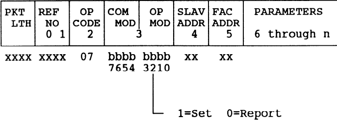
Figure 5 – Command packet for operating mode
