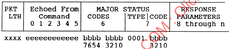
Figure 16 - Response packet for read
