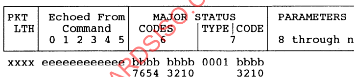
Figure 2 – Response packet for attributes
