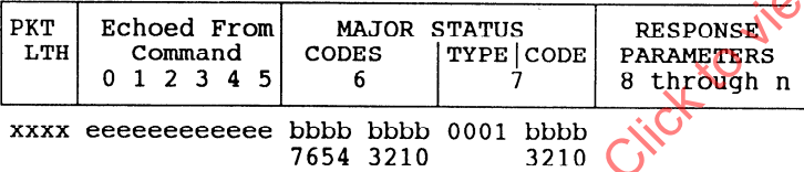
Figure 24 – Response packet for read from buffer
