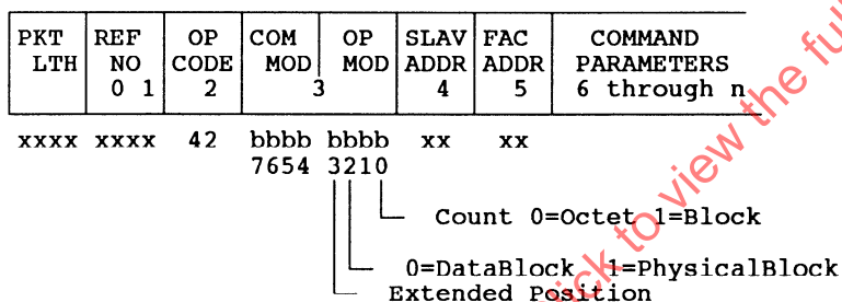
Figure 11 – Command packet for report position
