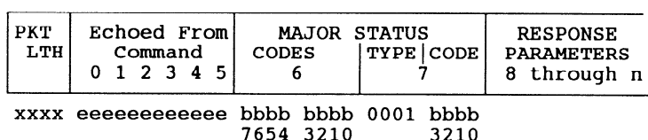
Figure 18 – Response packet for read raw data
