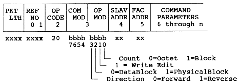
Figure 19 – Command packet for write
