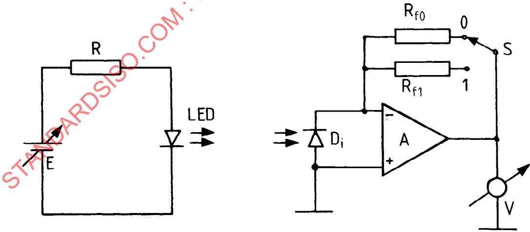
Figure B.2 - Electronic circuitry
