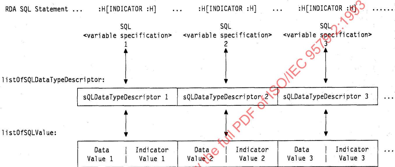
Figure 1 — Usage of Embedded SQL Variables
