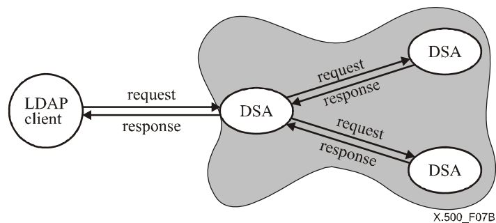
Figure 7b – Multi-chaining
