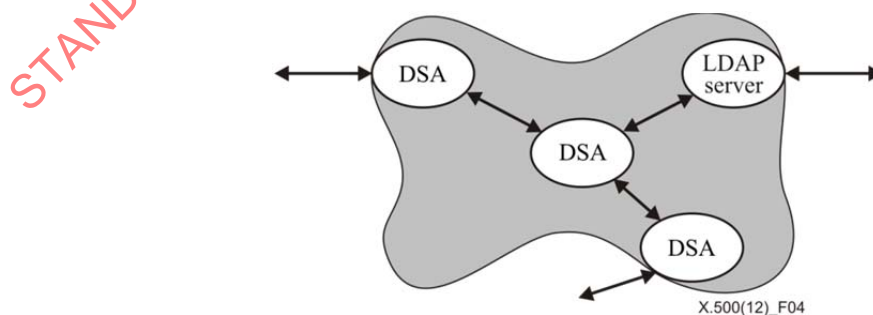
Figure 4 – Functional model of the Directory
