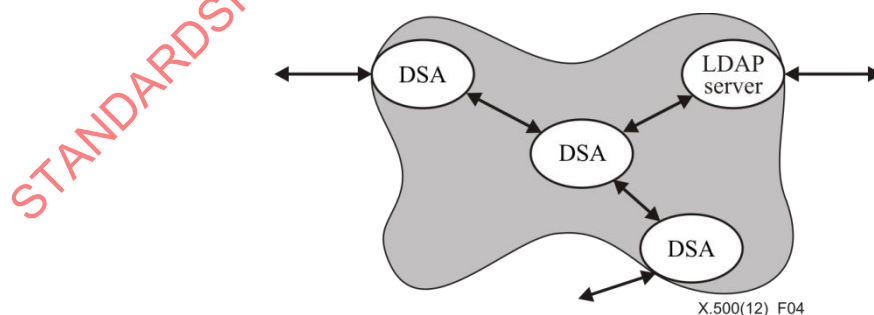
Figure 4 – Functional model of the Directory
