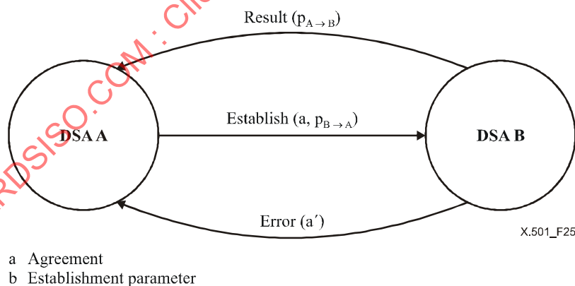
Figure 25 – DSA with Role A initiating establishment
