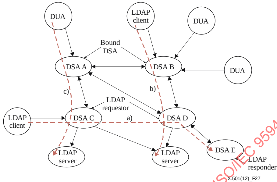
Figure 27 – LDAP interworking scenarios
