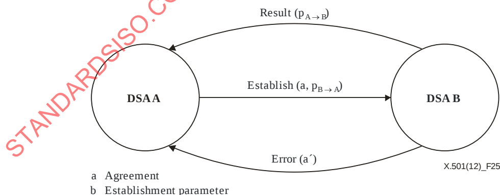
Figure 25 – DSA with Role A initiating establishment
