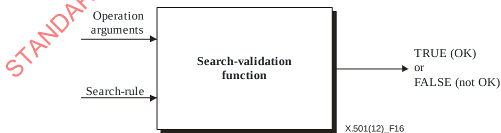
Figure 16 – Search-validation function
