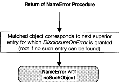
Figure B.2 – Return of Name Error
