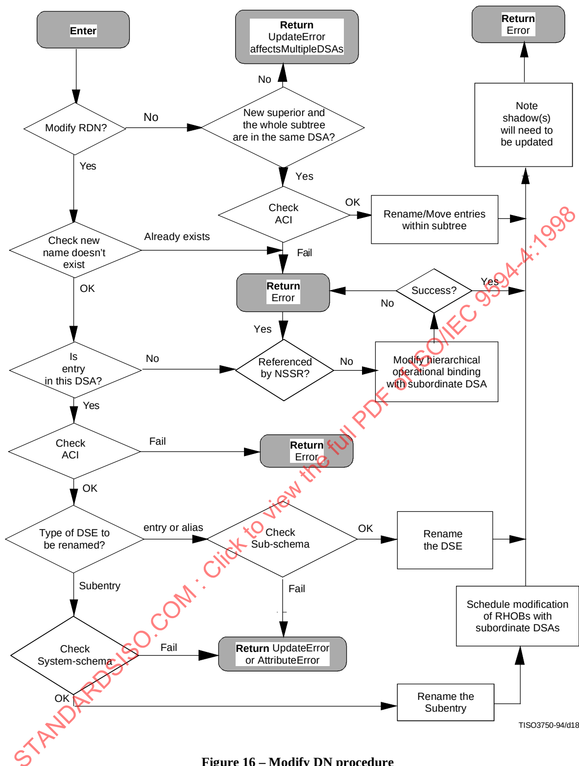
Figure 16 – Modify DN procedure
