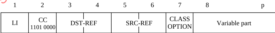
Figure 7 – Connection confirm (CC TPDU)
