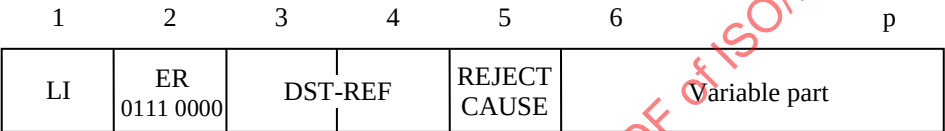
Figure 12 – Error TPDU
