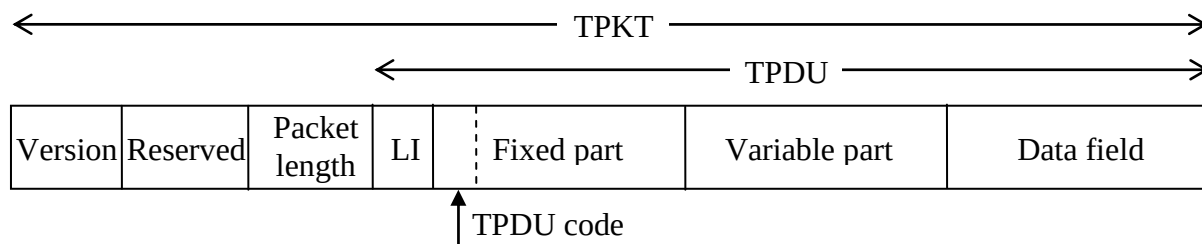
Figure 4 – TPKT structure
