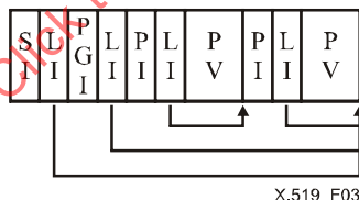
Figure 3 – SPDU with parameters – Grouped
