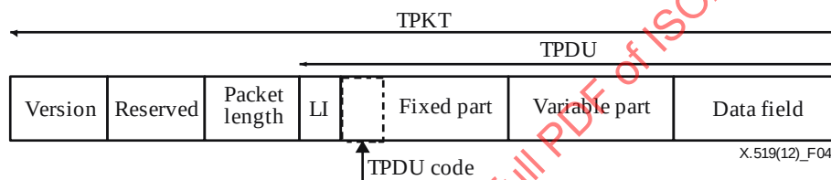
Figure 4 – TPKT structure
