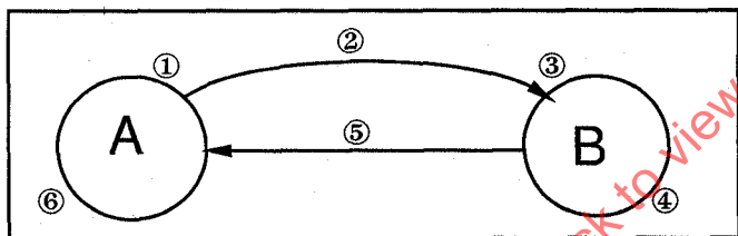
Figure 8 — Two-way Authentication
