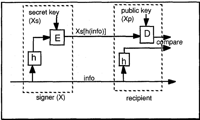
Figure 6 — Digital Signatures
