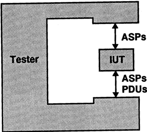
Figure 6 - Conceptual Testing Architecture
