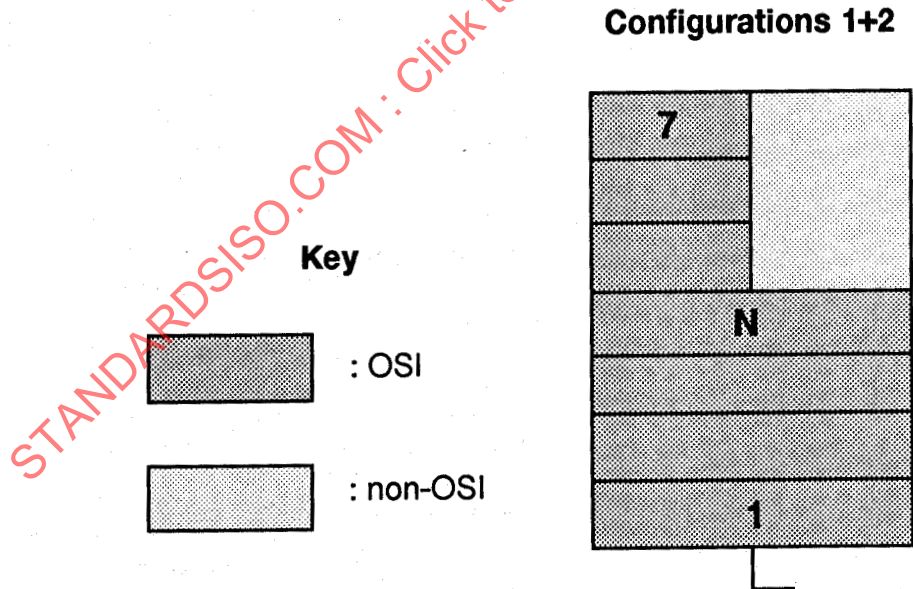
Figure 5 - Combination of 7-layer and partial (N)-open systems
