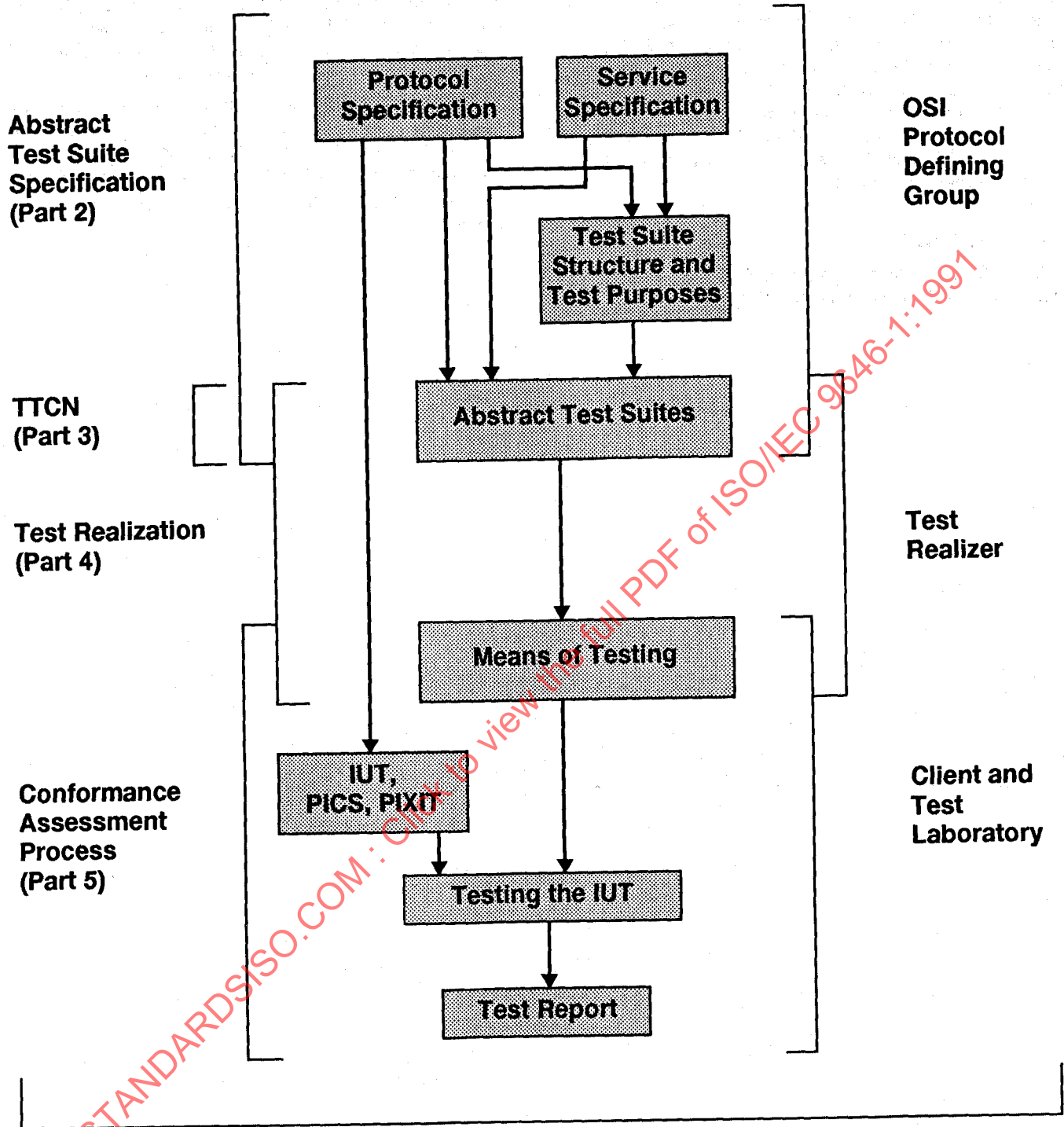
OSI Conformance testing methodology General concepts (Part 1)
