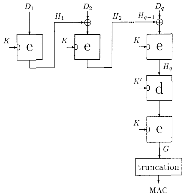
Figure 4 — MAC Algorithm 3.
