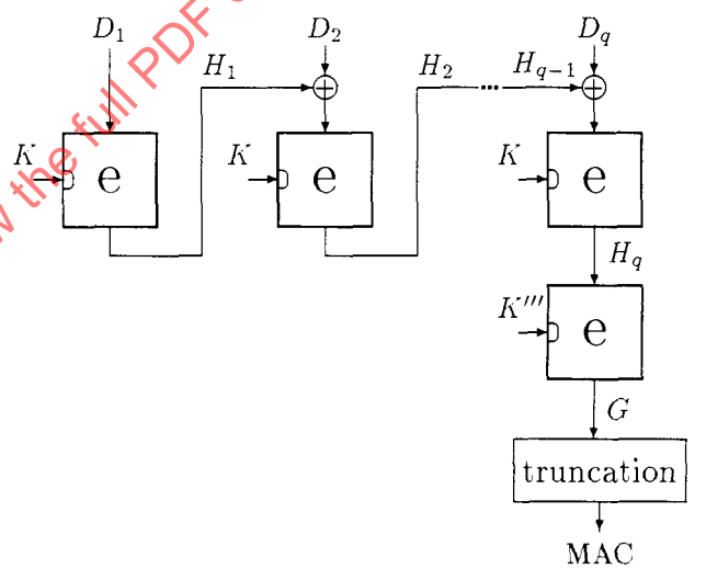
Figure 3 — MAC Algorithm 2.
