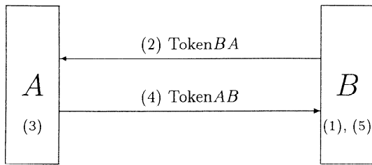
Figure 3 — Trusted public transformation based mechanism
