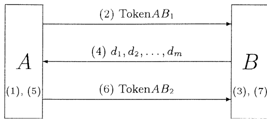
Figure 1 — Identity-based mechanism
