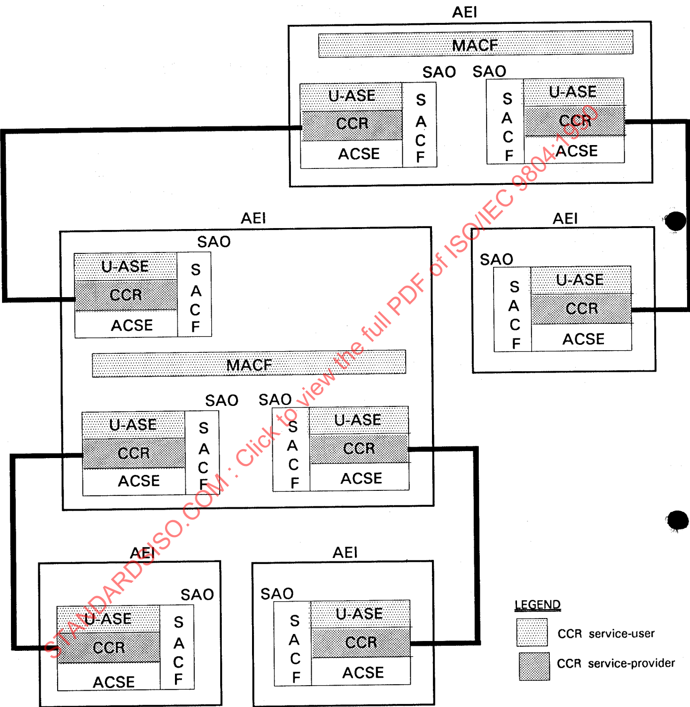
Figure B.1 Atomic action tree architecture
