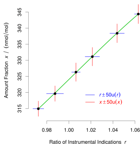
Figure 6: Analysis function used to assign values to the amount fraction of \text{N}_2\text{O} in a southern oceanic air reference material. The coordinates of the black dots are ratios and amount fractions for the primary calibration standards
