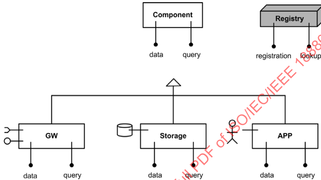
Figure 3—UGCCNet system model
