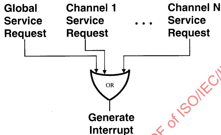
Figure 11 — Interrupt generation
