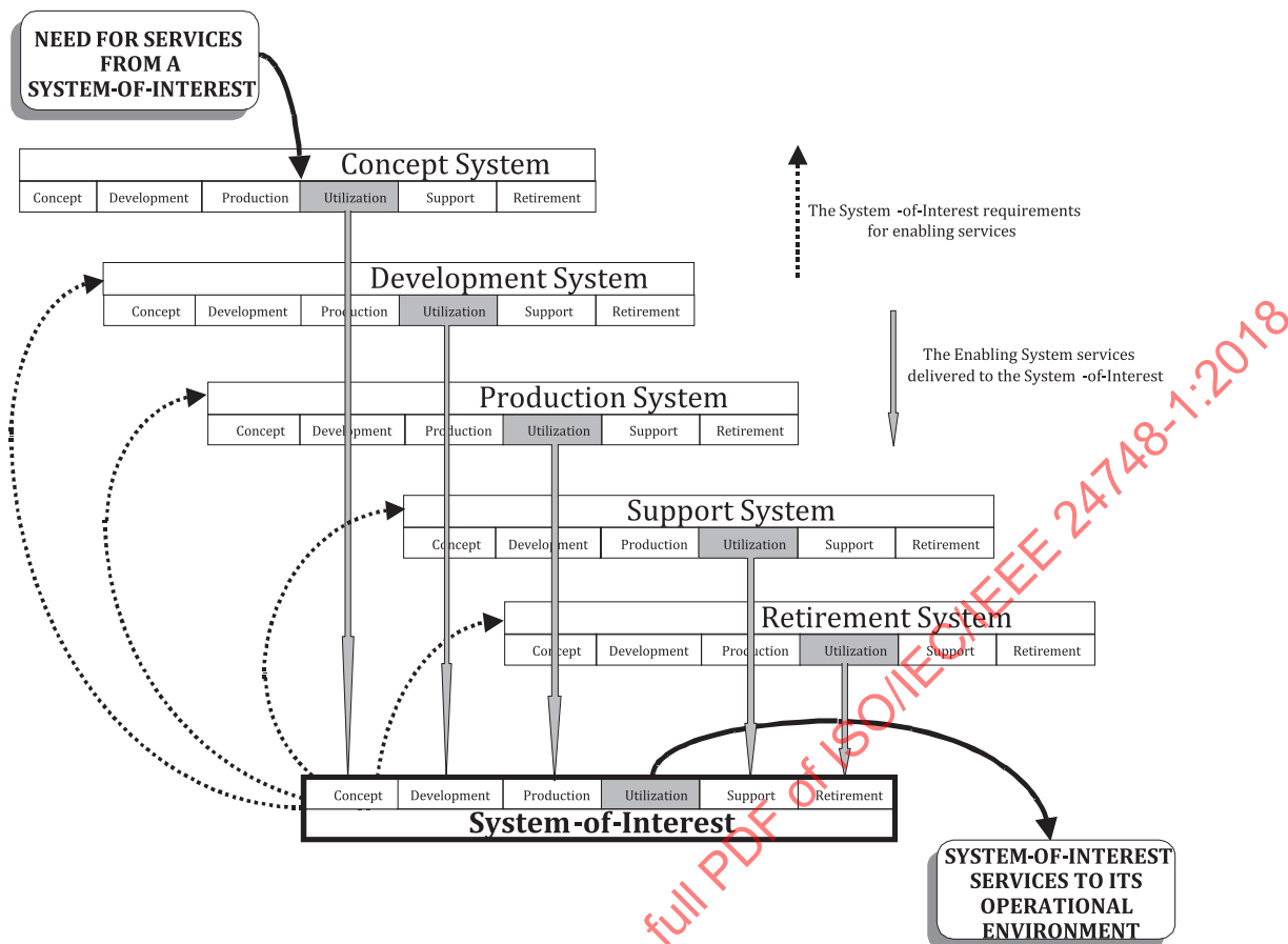
Figure 7 — System interaction with typical enabling systems
